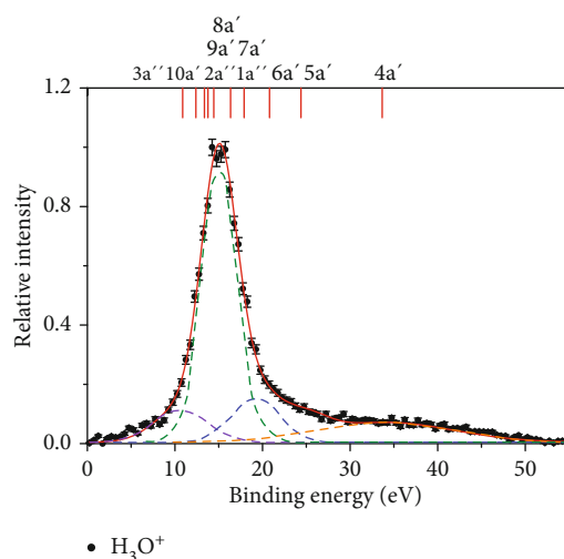
FIGURE 3: The same as Figure 2 but for \text{H}_3\text{O}^+ .
