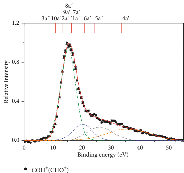
FIGURE 2: The binding energy spectrum for the formation of the \text{COH}^+ cation. The dashed lines are Gaussian fits, while the red solid curve is the sum of the Gaussians.
