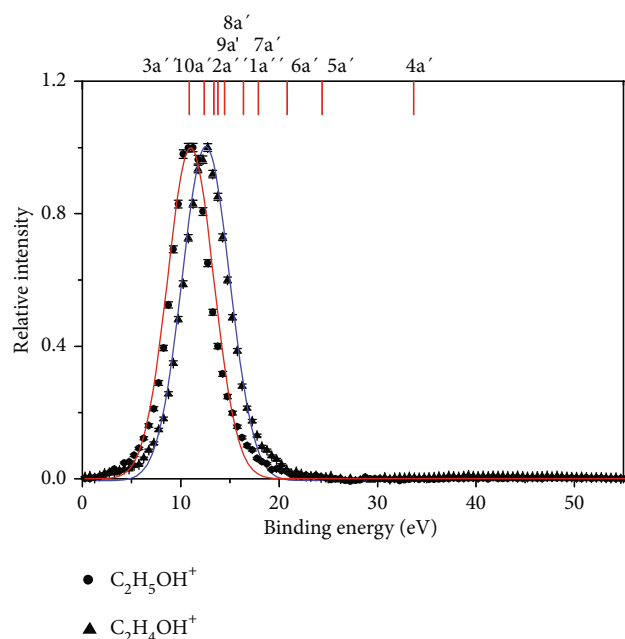
FIGURE 1: The binding energy spectra related to the \text{C}_2\text{H}_5\text{OH}^+ and \text{C}_2\text{H}_4\text{OH}^+ cations. The black solid circles and the black solid triangles with error bars represent the experimental data of \text{C}_2\text{H}_5\text{OH}^+ and \text{C}_2\text{H}_4\text{OH}^+ , respectively. The data for both ions are normalized to unity at the maximum. The red and blue solid curves are Gaussian fits. At the top of the plot, red solid vertical lines indicate the ionization energies of valence orbitals [32].
