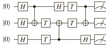
Figure A.1 Example of a quantum circuit with gates drawn from the Clifford + T gate set. Time flows from left to right. The two qubit gates are CNOT gates with the control indicated by the symbol • and the target indicated by the symbol \oplus .
