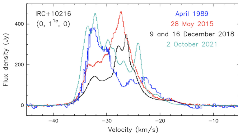
Figure 2. Observed variability of the HCN (0,1^e,0) J=2-1 maser at 177.2 GHz in the carbon star IRC+10216. The different colored lines show the results from different observing dates. From Jeste et al. (2022) .
