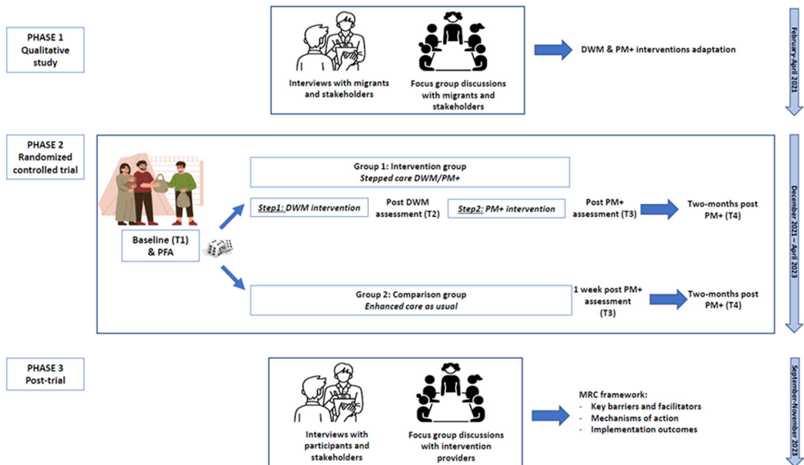
Figure 1. Trial phases.
