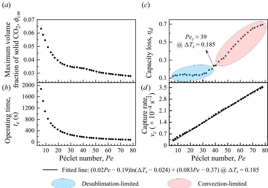
Figure 15. Analyses of CO 2 capture performance in packed-bed tests with the subcooling degree \Delta T_s = 0.185 and the Peclet numbers Pe \in [6.23, 77.84] . (a) The maximum volume fraction of solid CO 2 ( \phi_{cm} ) captured by the bed. (b) The operating time for CO 2 desublimation and sublimation ( t_e ). (c) The CO 2 capacity loss due to the time delay between the maximum point and the saturation point ( \eta_d ). (d) The CO 2 capture rate ( v_c ).
