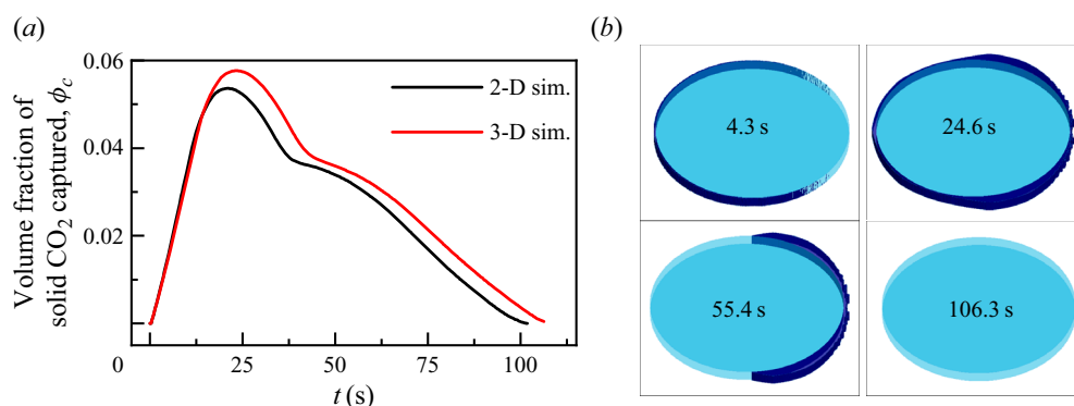
Figure 22. Comparison between 2-D and 3-D simulations. Temporal evolutions of (a) volume fraction of the captured solid CO 2 ( \phi_c ) and (b) contours of solid CO 2 .
