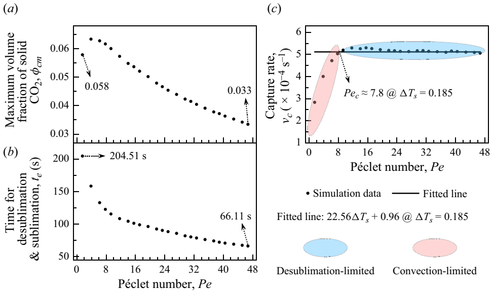
Figure 8. Analyses of CO 2 capture performance in single-grain tests with the subcooling degrees \Delta T_s = 0.185 and the Péclet numbers Pe \in [1.55, 46.70] . (a) The maximum volume fraction of solid CO 2 ( \phi_{cm} ) captured by the grain. (b) The operating time for CO 2 desublimation and sublimation ( t_e ). (c) The CO 2 capture rate ( v_c ).
