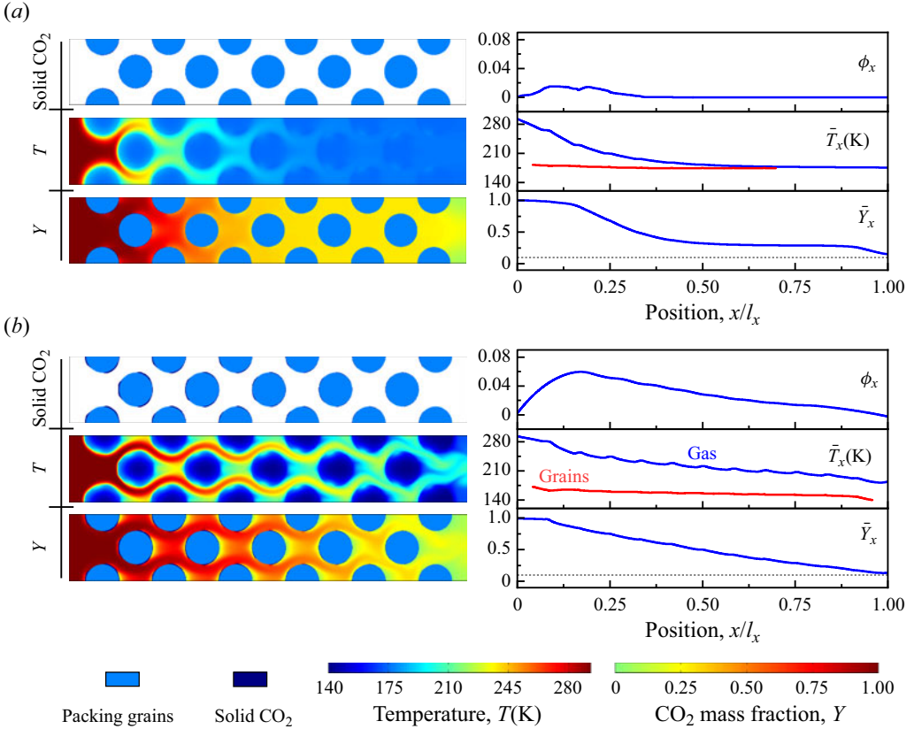
Figure 16. The CO 2 desublimation and sublimation properties in a packed bed. Contours of solid CO 2 , temperature ( T ), CO 2 mass fraction ( Y ) and the corresponding vertically averaged profiles in (a) the test with the subcooling degree \Delta T_s = 0.006 and the Péclet number Pe = 15.57 at t = 6.20 s, and (b) the test with the subcooling degree \Delta T_s = 0.185 and the Péclet number Pe = 77.84 at t = 8.67 s.
