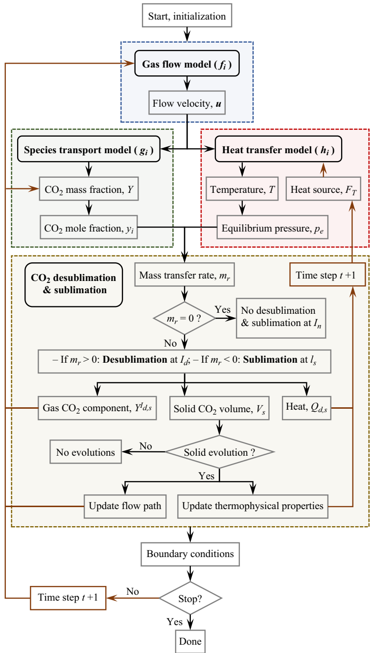
Figure 3. The schematic diagram of the overall numerical implementation.
