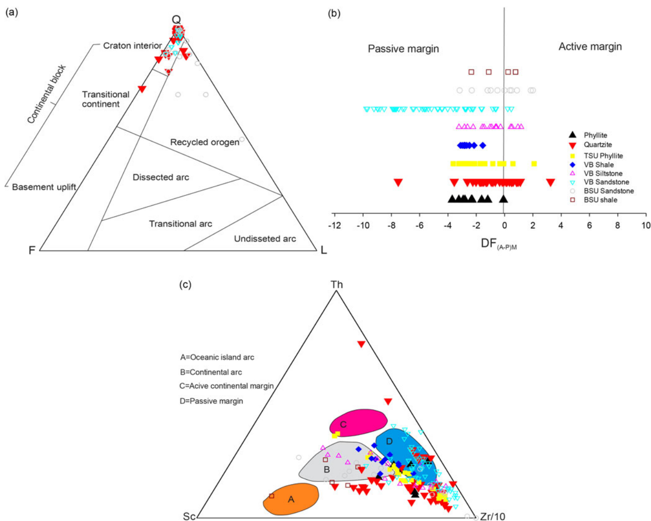
Figure 11. Tectonic setting discrimination diagrams for the rocks of the TSU (a) Q-F-L diagram (Dickinson et al. , 1983), (b) DF(A-P)M diagram (after Verma and Armstrong-Altrin, 2016) and (c) Th-Sc-Zr/10 plot (Bhatia and Crook, 1986). The TSU data are compared to published data from the sandstones and shales of the Buem structural unit, Kwahu-Bombouaka Group of the Voltaian Supergroup and phyllites from the TSU (Osae et al. , 2006; Kalsbeek and Frei, 2010; Abu and Zongo, 2017; Anani et al. , 2017, 2019; Amedjoe et al. , 2018; Abu et al. , 2020). DF = Discriminant function, A and P are active and passive margin, respectively, and M = major element composition.
