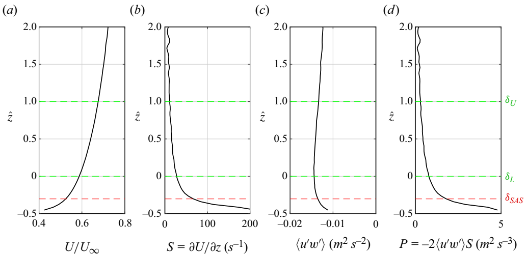
Figure 10. For the SDSL TBL case, the wall-normal profiles of (a) normalised mean velocity, (b) mean shear rate, (c) Reynolds shear stress and (d) turbulence production rate. The horizontal lines indicate \delta_U , \delta_L and \delta_{SAS} , as labelled in the figure.
