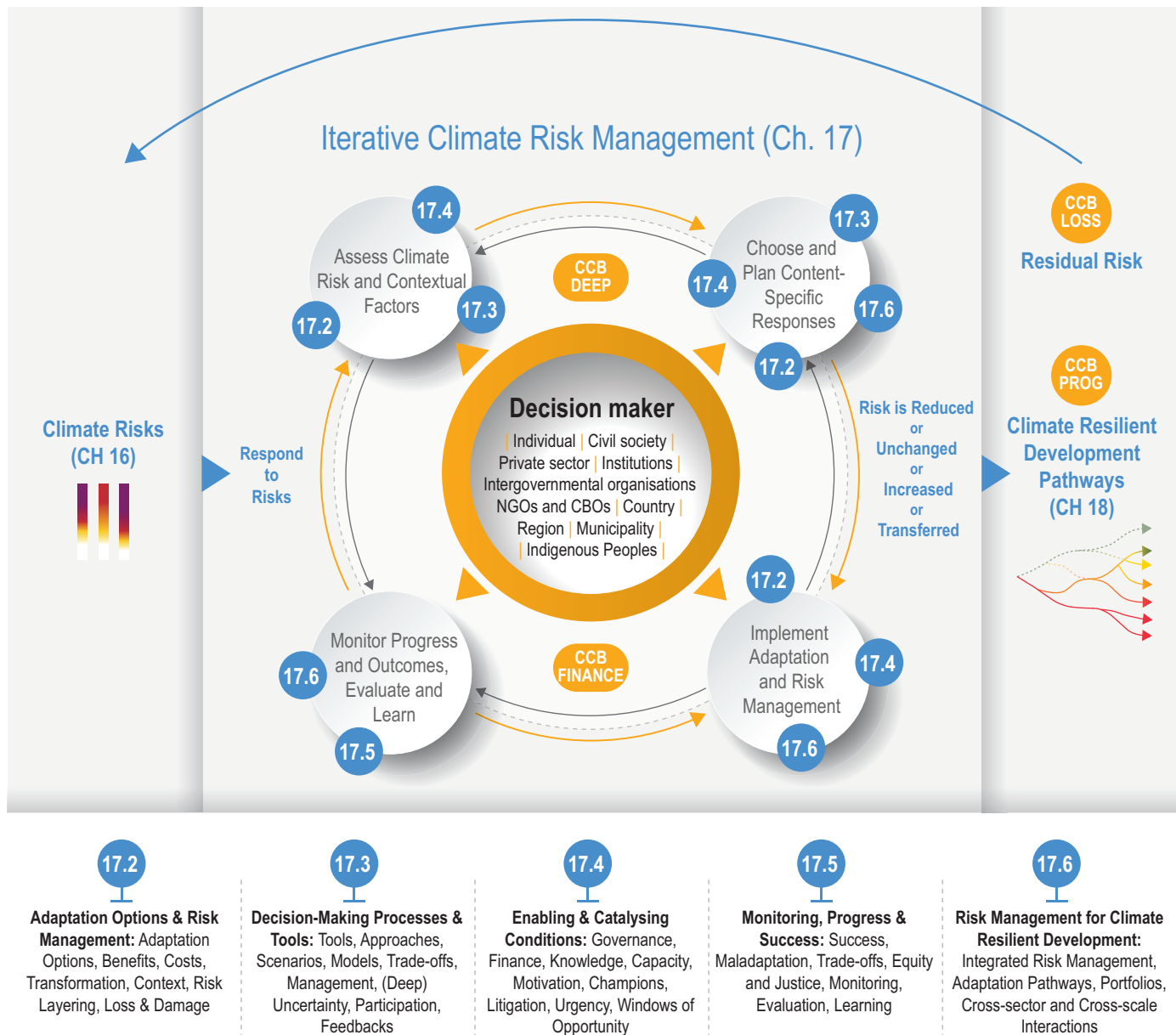
Figure 17.1 | Schematic representation of the climate risk management decision-making process as introduced in Chapter 1 (Figure 1.6) and the key elements of this chapter that address additional aspects of this process. In Chapter 17, climate risk management (middle box) is framed as the iterative response (i.e., what society could do and how it could be done) to the climate risks described in Chapter 16, with outcomes (ideally reduced risk) that can support (or perhaps hinder) climate resilient development, as assessed in Chapter 18. Decision makers from diverse contexts sit at the centre of the climate risk decision-making process and interact with and drive these processes as they play out. The main sections of Chapter 17 (bottom panel of boxes) address a wide range of issues (keywords in bottom panel) that manifest at one or more stages of climate risk management processes, illustrated by icons for section numbers and Cross-Chapter Boxes in the interactive risk management process.
