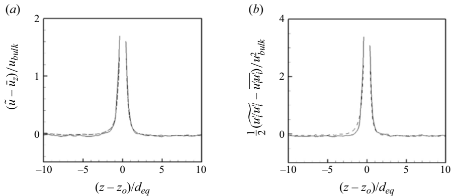
Figure 6. Axial profiles of the differences in the time-averaged and ensemble-averaged water flow variables near a bubble (case ML): (a) \tilde{u}_z - \bar{u}_z (axial velocity); (b) (\tilde{u}_i' u_i' - \overline{u_i' u_i'})/2 (turbulent kinetic energy); —, r_o/R = 0.5 ; - - -, r_o/R = 0.89 .
