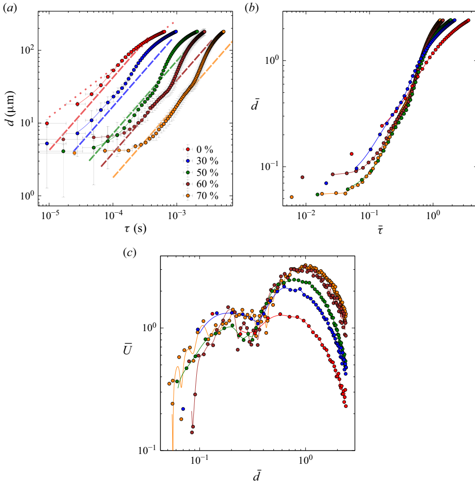
Figure 5. Influence of viscosity on the dynamics of the capillary bridge on the PDMS@Au surface ( Oh = 0.005–0.12 .) (a) Minimum width versus time before breakup. The dashed lines represent power laws with a power of one, where the prefactor for the 70 % liquid is 1.78 \text{ cm s}^{-1} , and the prefactors for the remaining cases are calculated accordingly (see § 3.2.2). The error bars represent the standard deviation of at least four experiments. (b) Scaled minimum width versus scaled time before breakup. The minimum width is normalised with the minimum width at maximum velocity of the 70 % ( a_m ) liquid. The time before breakup is normalised with \zeta_{tot} a_m / \gamma . (c) Scaled breakup velocity versus scaled minimum width. The breakup velocity is scaled with \gamma / \zeta_{tot} . The legend of panel (a) applies to all panels. Due to the loss of resolution of the imaging system, less emphasis should be put on d \leq 8 \text{ } \mu\text{m} .
