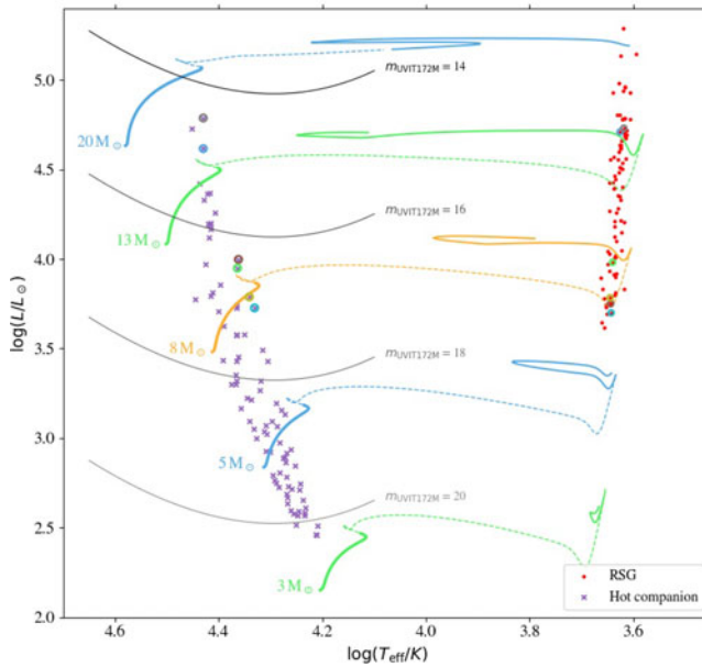
Figure 1. Hertzsprung–Russell diagram showing the RSGs and their companions. The coloured lines show stellar evolutionary tracks that are based on those in Schootemeijer et al. (2019). The solid grey lines highlight lines of constant UVIT magnitudes in the stellar models. Rings of different colours highlight the six systems that have a mass-ratio greater than 1.
