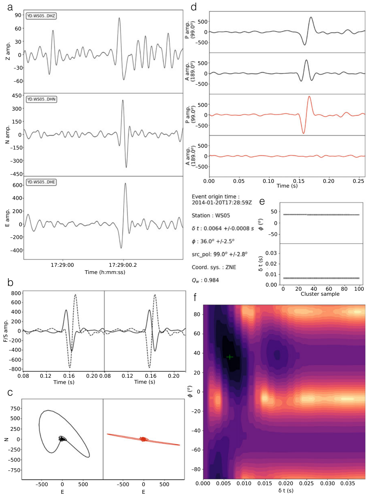
Figure 2. An example of a well-constrained shear-wave splitting event. (a) Icequake signal before correction in the vertical, north and east component. (b) The waveforms before (left) and after (right) SWS correction, plotted in the fast (black line) and slow (dotted) directions. (c) Horizontal (north and east) particle motion before (left) and after (right) SWS correction. (d) Particle motion of icequakes in the source polarisation (P) and the perpendicular azimuth (A) before (top two) and after (bottom two) correction. (e) Optimal \phi and \delta t for different cluster sizes. A good splitting measurement should have constant \phi and \delta t values independent of cluster size. (f) Error surface plotted on \phi vs \delta t . Larger errors are represented with brighter colours, and smaller errors with darker colours. The optimal \phi and \delta t and its uncertainties are shown with the green symbol.
