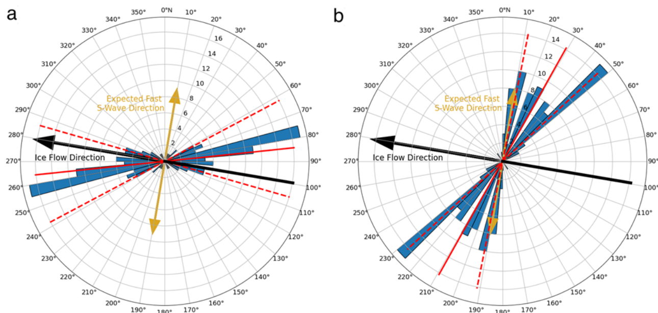
Figure 3. Rose diagrams of (a) source polarisations and (b) fast S-wave directions for all the 80 SWS measurements. The solid and dotted red lines indicate the averages and uncertainties respectively. The gold arrows on both diagrams indicate the expected fast S-wave direction based on ice flow direction, which are shown as black arrows (see main text for further details). Method for estimating uncertainty is included in the supplementary information.
