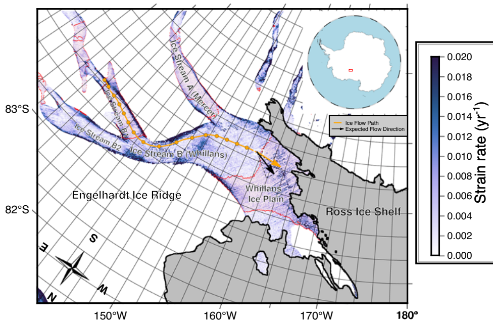
Figure 4. A summary of the study findings. Regions with a flow direction between 281^{\circ}\text{N} and 317^{\circ}\text{N} are shaded in red. The orange arrow shows the present-day flow direction. The black arrow indicates the flow direction inferred from the fast S-wave polarisation direction, and the dashed black sector outline shows the range of azimuths expressed by the red shaded regions. The background colour map is the strain rate calculated using the velocity map of Rignot and others (2017, supplementary information for calculation). Other features shown in this map are as in Figure 1a. The azimuth of the strain rate is shown in Figure S3.
