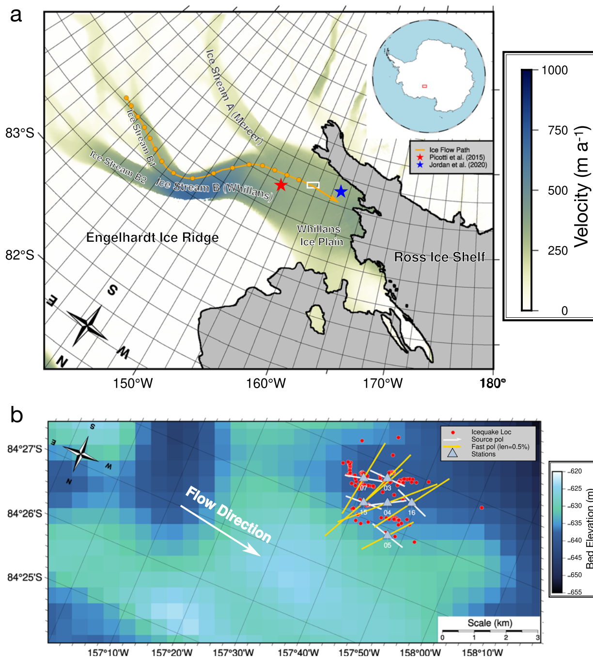
Figure 1. Stereographic maps showing Whillans Ice Stream (WIS) and study location. (a) Regional map of the WIS. The grounding line is marked in the thick black line, and the grey shaded areas mark regions of floating ice. The blue and red star show the study site locations of Jordan and others (2020) and Picotti and others (2015), respectively. The orange line outlines the upstream flow path of the ice at our study site location, assuming current flow velocities, with orange points marking the locations at intervals of 50 years (see supplementary information for flow path calculation). The background colour map shows the ice flow velocity obtained from MEaSUREs InSAR-Based Antarctica Ice Velocity Map, Version 2 (Rignot and others, 2017). The study area in (b) is outlined by the white box. (b) Detailed map of the study region. Stations are marked as blue triangles, and icequake locations are shown by red scatter points. Gold lines show the fast S-wave polarisation direction, with the length of the line representing the strength of anisotropy. White lines show the source polarisations for each event, as estimated from recorded shear waves. Dominant ice flow direction ( 280^\circ ) is indicated by the large white arrow. The background colour map shows the bed elevation (Morlighem, 2022).
