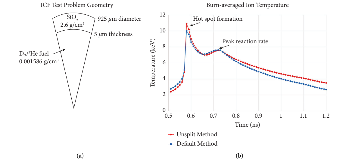
FIGURE 7: An ICF test problem based on an OMEGA capsule experiment: (a) the initial geometry of the capsule and (b) the calculated burn-averaged ion temperature from separate highly resolved 1D simulations using the default and unsplit hydrodynamic methods in xRAGE.
