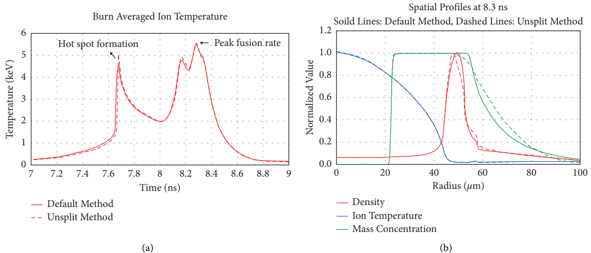
FIGURE 12: Results from highly resolved 1D simulations of the indirect drive ICF problem at 0.25\ \mu\text{m} uniform spatial resolution: (a) burn-averaged ion temperature during formation of the hot spot and (b) spatial profiles at 8.3 ns of density normalized by 380\ \text{g/cm}^3 , ion temperature normalized by 8\ \text{keV} , and cryogenic layer mass concentration.
