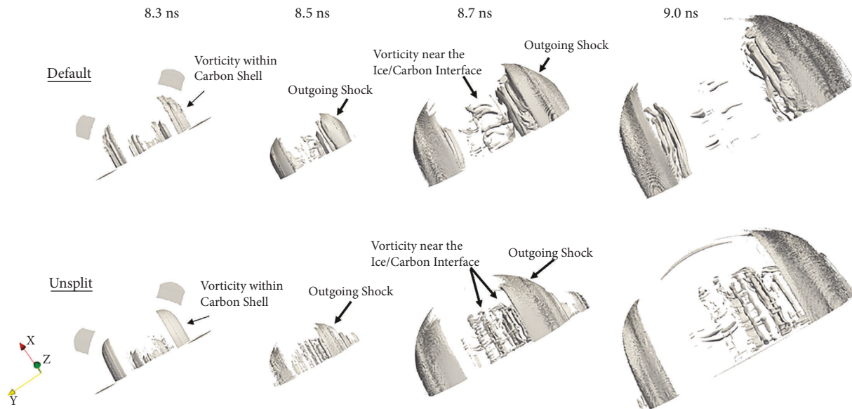
FIGURE 15: Isosurfaces where the Q-criterion is equal to 10^{18}\text{s}^{-2} at four different times within a 256\mu\text{m} by 512\mu\text{m} by 256\mu\text{m} sized box region for the indirect drive ICF test problem using both the default and unsplit methods. The spatial resolution within the box region is 0.5\mu\text{m} .
