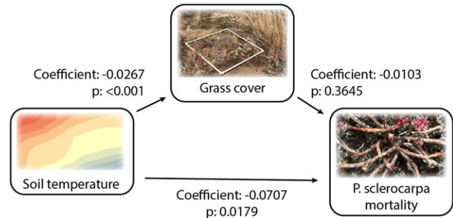
Fig. 3. Diagram representing the structural equation model implemented. The model included Portulaca sclerocarpa mortality from 2017 to 2021 as the dependent variable, invasive grass cover as an endogenous variable affecting P. sclerocarpa mortality and soil temperature as an exogenous variable affecting both invasive grass cover and P. sclerocarpa mortality. Photographs: Nathan S Gill, Hawai'i Volcanoes National Park, 2017.
