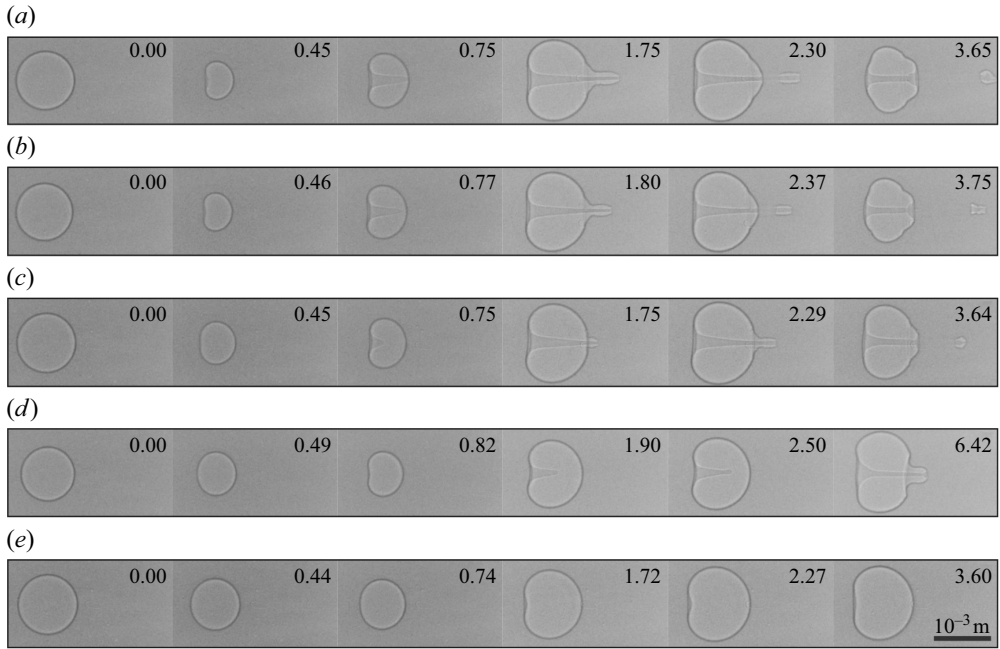
Figure 2. Image sequence of the dynamics of an air bubble interacting with a shock wave travelling from left to right, of dimensionless pressure impulse of J/(r_0^3 \sqrt{p_{b,0} \rho}) : (a) 10.40, (b) 8.62, (c) 6.72, (d) 5.03 and (e) 3.48. The dimensionless time, t/(r_0 \sqrt{\rho/p_{b,0}}) , is indicated on each frame and zero is the time at which the shock contacts the bubble. The scale bar is the same for all image sequences.
