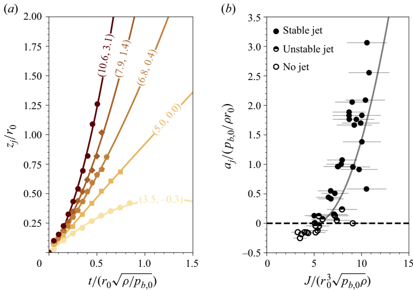
Figure 4. (a) Time evolution of the jet tip location during the bubble collapse. The dimensionless impulse and acceleration of the jet are indicated in brackets for each curve [J/(r_0^3 \sqrt{\rho p_{b,0}}), a_j/(p_{b,0}/\rho r_0)] . (b) Dimensionless acceleration of the jet tip during the collapse phase of the bubble against the dimensionless pressure impulse of the shock wave applied to the bubble surface. The dashed dark line indicates the jetting limit for a_j/(p_{b,0}/\rho r_0) \approx 0 and the grey curve shows the scaling law in (3.4).
