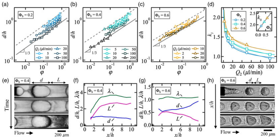
Figure 4. Droplet formation at low \varphi . Flow rates in \mu\text{l/min} . (a) Evolution of d/h as a function of \varphi for \Phi_S = 0.2 . Solid line: d/h = 0.95\varphi^{1/3} . Dashed line: d/h = 1.67\varphi^{1/3} . (b) Variation of droplet size with flow rate ratio for \Phi_S = 0.4 . Solid line: d/h = 0.91\varphi^{1/3} . Dashed line: d/h = 1.68\varphi^{1/3} . (c) Droplet size d/h versus \varphi for \Phi_S = 0.6 . Solid line: d/h = 1.3\varphi^{1/3} . Dashed line: d/h = 1.9\varphi^{1/3} . (d) Role of flow rate Q_2 on prefactor k_J for \Phi_S = 0.2 ( \circ ), 0.4 ( \square ) and 0.6 ( \triangle ). Solid lines: k_J = k_0 Q_2^{-0.15} . Inset: k_0 versus \Phi_S . Solid line: k_0 = 1.8\Phi_S^{0.87} . (e) Time series of micrographs in the droplet reference frame at \Phi_S = 0.4 for (Q_1, Q_2) = (3, 5) , \Delta t = 2 s. (f) Spatial evolution of d/h , L/h , and \lambda/h at \Phi_S = 0.4 for (Q_1, Q_2) = (1, 10) . (g) Flow spatial evolution at \Phi_S = 0.6 for (Q_1, Q_2) = (1, 10) . (h) Micrograph showing spatial evolution of droplet microflows at \Phi_S = 0.6 for (Q_1, Q_2) = (1, 10) , \Delta x/h \sim 3 .
