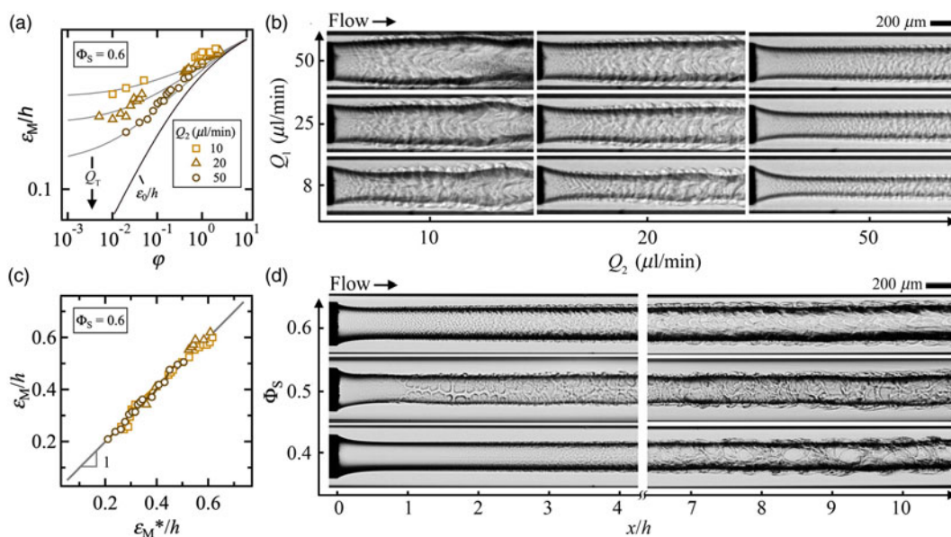
Figure 10. Jets at moderate and large solvent concentrations \Phi_S . (a) Evolution of iso- Q_2 curves of minimum jet diameter \varepsilon_M/h as a function of flow rate ratio \varphi at \Phi_S = 0.6 . Solid lines: Eq. (6.2) with Q_T = Q_1 + Q_2 . (b) Chart of jet micrographs near the fluid contactor at \Phi_S = 0.6 . (c) Comparison of measured \varepsilon_M/h with predicted \varepsilon_M^*/h . Solid line: \varepsilon_M/h = \varepsilon_M^*/h . (d) Micrograph showing the influence of solvent concentration on upstream and downstream jet morphology at \varphi = 1 with Q_1 = Q_2 = 100 \mu\text{l/min} for all fluids.
