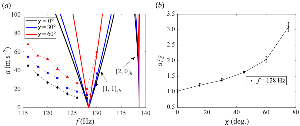
Figure 15. (a) Instability tongue for the mixed mode plotted in the acceleration–frequency ( A-\omega ) space. Experimental data are given by the symbols. Theoretical predictions are shown in solid lines for the subharmonic [1, 1] rocking mode and harmonic [2, 0] pumping mode for \alpha = 60.7^\circ and V = 4.6 ml with pinned contact line. (b) Threshold acceleration a/g against slanting angle \chi at the resonance frequency f = 128 Hz.
