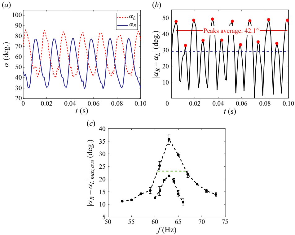
Figure 11. Procedure for obtaining the harmonic frequency response curve by measuring the time trace of (a) the dynamic contact angles at two sides of the drop, \alpha_L , \alpha_R , for a = 0.25 g, f = 63 Hz and \chi = 60^\circ . (b) The difference in contact angles |\alpha_R - \alpha_L| is used as a metric for the frequency response, where the red dots denote the peak points of the signal, and the red line is the average value of these points, while the dashed blue line represents the overall average. (c) Frequency response curve plotting |\alpha_R - \alpha_L| against driving frequency f for two different slanting angles, \chi = 30^\circ (squares) and \chi = 60^\circ (circles). The green dashed line corresponds to 65 % of the peak value of the response curve at \chi = 60^\circ .
