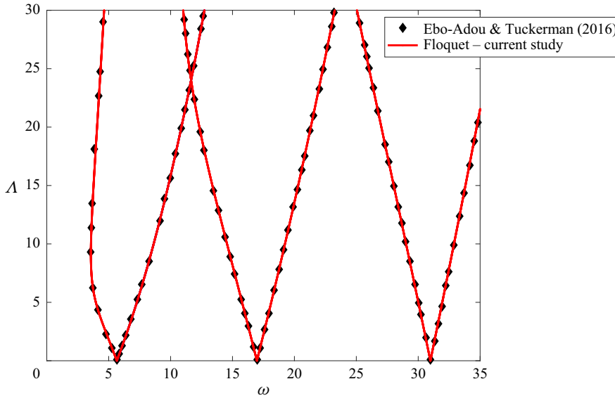
Figure 4. Verification of Floquet theory for sessile drops with radial forcing. Subharmonic instability tongues for the [2, 0] , [4, 0] , [6, 0] hemispherical sessile drop modes with free contact line compared with those predicted by Ebo-Adou & Tuckerman (2016) for the full spherical drop.
