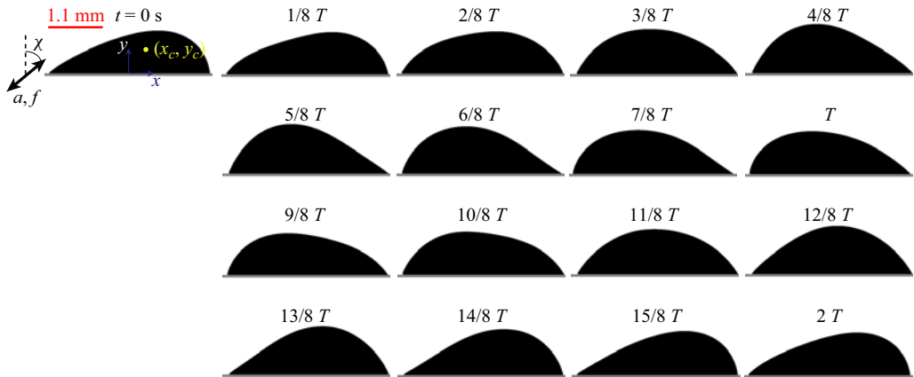
Figure 13. Mixed mode excited with a = 2.2g , f = 128 Hz, \chi = 60^\circ , \alpha = 60.7^\circ and V = 4.6 ml. The period of the substrate oscillation is T , whereas the period of the drop oscillation is 2T .
