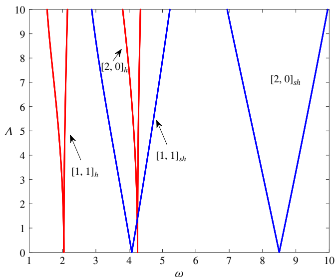
Figure 2. Typical instability tongues for the [1, 1] and [2, 0] modes plotted in the acceleration–frequency ( \Delta – \omega ) space. Here, the contact line is pinned, the slanting angle is \chi = 30^\circ , and the contact angle is \alpha = 90^\circ .
