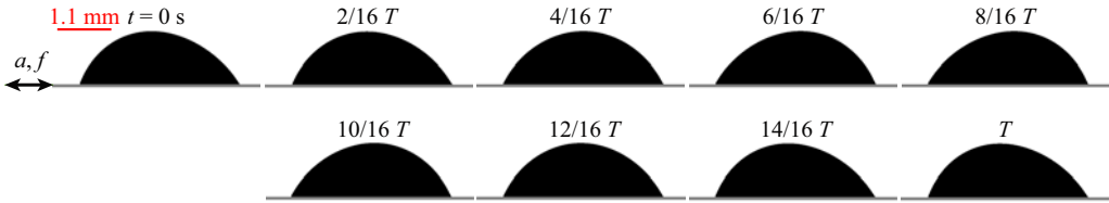
Figure 10. Harmonic rocking mode [1, 1] over a complete cycle of oscillation with period T , which has been excited at acceleration a = 0.25 g and frequency f = 63.5 Hz using horizontal \chi = 90^\circ vibration, with contact angle \alpha = 60.7^\circ and volume V = 4.6 ml.
