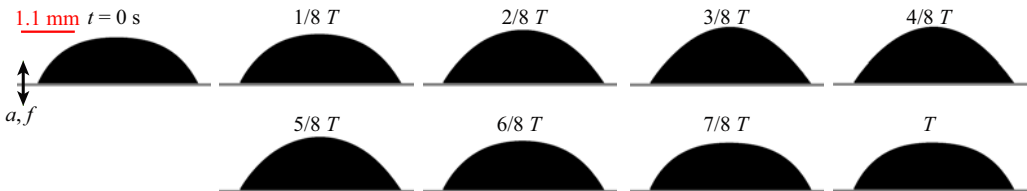
Figure 9. Harmonic pumping mode [2, 0] over a complete cycle of oscillation with period T , which has been excited at acceleration a = 0.25 g and frequency f = 128 \text{ Hz} using vertical \chi = 0^\circ vibration, with contact angle \alpha = 60.7^\circ and volume V = 4.6 \text{ ml} .
