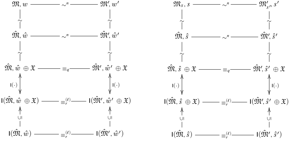
FIGURE 4. Upgrading for relational epistemic models, refined by Proposition 3.7.
