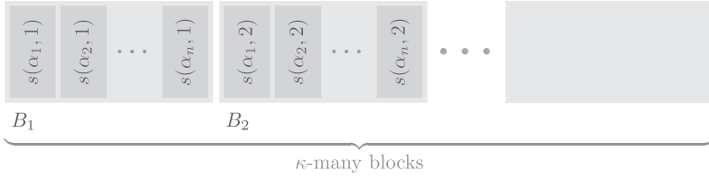
FIGURE 5. Subdivision of [w]_a = \sigma_a(w) in the local a -structure \mathbb{M} \upharpoonright [w]_a for an inquisitive assignment \Pi = \Sigma_a(w) that is \kappa -regular at granularity m , where \rho_m(\Pi \setminus \emptyset) = \{\alpha_1, \alpha_2, \dots, \alpha_n\} , \kappa = \{1, 2, \dots\} and each one of the contributions s(\alpha_j, i) in block B_i is one \subseteq -maximal element in \Pi , so that there are precisely \kappa many such for each available \sim^m -type of nonempty information states in \Pi .
