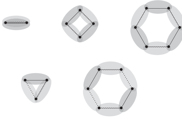
FIGURE 6. Example of particularly simple unfoldings in bisimilar coverings of S5 Kripke frames for agents with wavy , straight , dotted accessibility edges, respectively, and different shades for corresponding equivalence classes; top row: unfolding of a 2-cycle (overlap of two equivalence classes in two worlds) into a 4- or 6-cycle; below: unfolding of a 3-cycle into a 6-cycle (just non-trivial equivalence classes indicated and worlds in overlaps and links in induced cycles marked).
