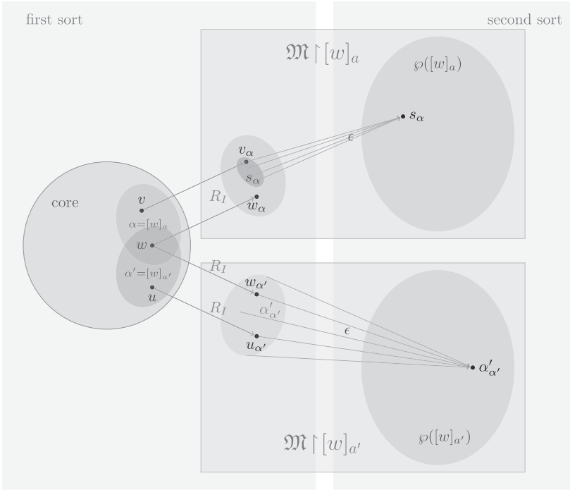
FIGURE 3. Structural layout of the exploded view I(\mathfrak{M}) of \mathfrak{M} ; selectively displayed are the representations of intersecting local structures \mathfrak{M} \upharpoonright [w]_a , \mathfrak{M} \upharpoonright [w]_{a'} w.r.t. agents a and a' , with one element each from their (full powerset) second sorts. Here \alpha = [w]_a and \alpha' = [w]_{a'} contribute two overlapping local structures, whose disjoint (tagged) representations each contribute the full power set of their first sort to disjoint (tagged) representations in the second sort; displayed as particular elements of the second sort are s_\alpha for some s \subseteq \alpha (as part of the representation of the a -local structure \mathfrak{M} \upharpoonright [w]_a ) and the full set \alpha' \subseteq \alpha' (as part of the representation of the a' -local structure \mathfrak{M} \upharpoonright [w]_{a'} ).
