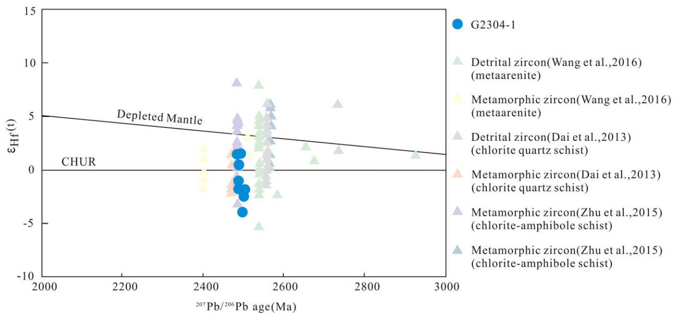
Figure 6. Zircon Age- \epsilon_{\text{Hf}}(t) diagram of meta-rhyolite in supracrustal rocks in the Anshan-Benxi area and supracrustal rocks in the Anshan-Benxi area of Zhu et al. , 2015, Dai et al. , 2013a and Wang et al. , 2016.
