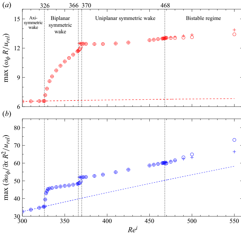
Figure 17. Maximum values of (a) the normalised azimuthal vorticity \omega_\phi (R/u_{rel}) and (b) its streamwise gradient \partial\omega_\phi/\partial x (R^2/u_{rel}) inside the droplet as a function of the internal Reynolds number for (\mu^*, Re^e) = (0.5, 200) . In both panels, coloured dashed lines denote results from an axisymmetric flow configuration. Circles: simulations starting from an initially axisymmetric flow; crosses: simulations starting from a uniplanar-symmetric flow corresponding to the fully developed state at Re^i = 450 .
