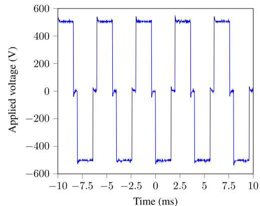
Figure 6. The bi-polar modulated voltage profile versus time, at a repetition rate of 0.5 kHz.
