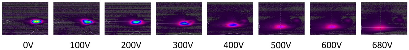
Figure 2. Beam deflection pictures at different voltages.
