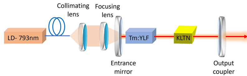
Figure 4. The system scheme of the actively Q -switched Tm:YLF laser based on an EO KLTN deflector.
