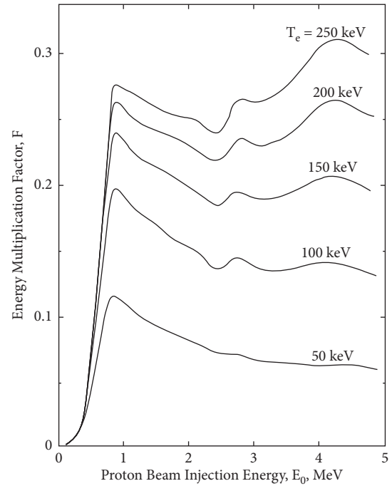
FIGURE 6: Energy multiplication factor vs proton injection energy for various electron temperatures. Protons are injected into a ^{11}\text{B} plasma with cold ions and warm electrons. The results are independent of plasma density when the value of \ln\Lambda is fixed. Reproduced from Moreau [9] with the permission of the publisher. © IAEA 1977.
