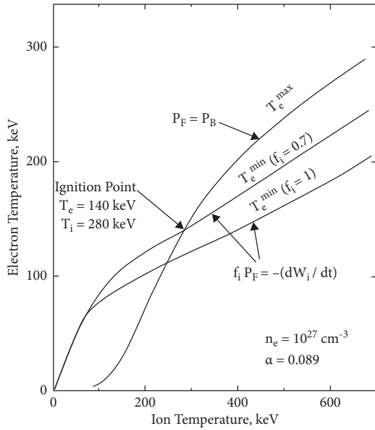
FIGURE 2: Ignition points in the T_e - T_i plane for high-density H- ^{11}\text{B} plasma. f_i is the fraction of fusion power to plasma ions; \alpha is the boron-to-proton ion concentration. Reproduced from Moreau [9] with the permission of the publisher. © IAEA 1977.
