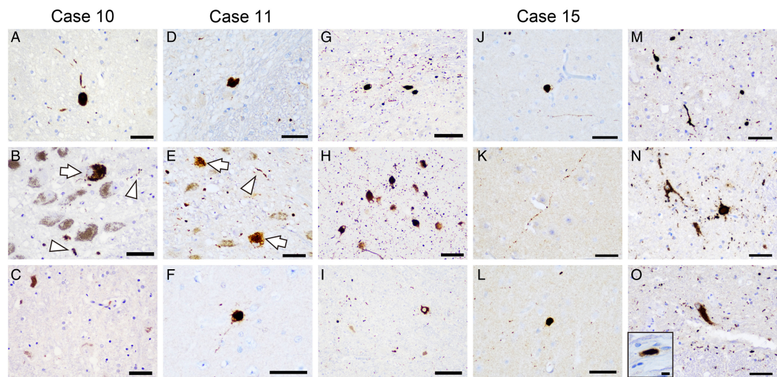
Figure 1: Representative microphotographs of alpha-synuclein pathology in the brain and spinal cord. a–o, Immunohistochemistry for alpha-synuclein (5G4). a–c, Case 10; d–f, case 11; g–i, case 15. a, d, g, Dorsal vagal nucleus in the medulla oblongata; b, e, h, locus coeruleus of the pons; c, i, substantia nigra in the midbrain; f, j, amygdala; k, CA2 in the hippocampus; l, anterior cingulate cortex; m, cervical spinal cord; n, thoracic spinal cord; o, lumbar spinal cord (inset: cauda equina). b, e, Arrows indicate neuronal cytoplasmic inclusion and arrowheads indicate Lewy neurites. Scale bar = 50 µm for a–f and j–o, 100 µm for g–i, and 10 µm for the inset of o.
