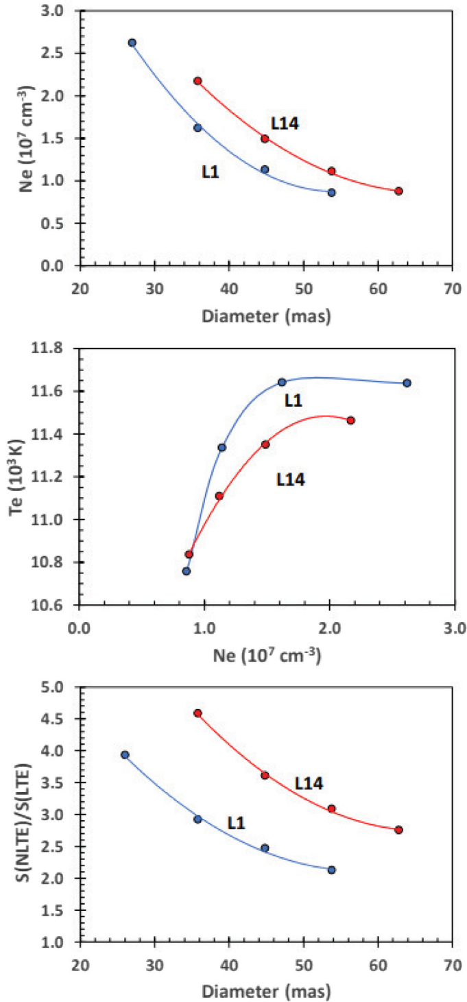
Figure 6. Physical conditions of the clumps that fit the spectra of the H30 \alpha recombination line of clumps 1 and 14, as identified in Figure 5.
