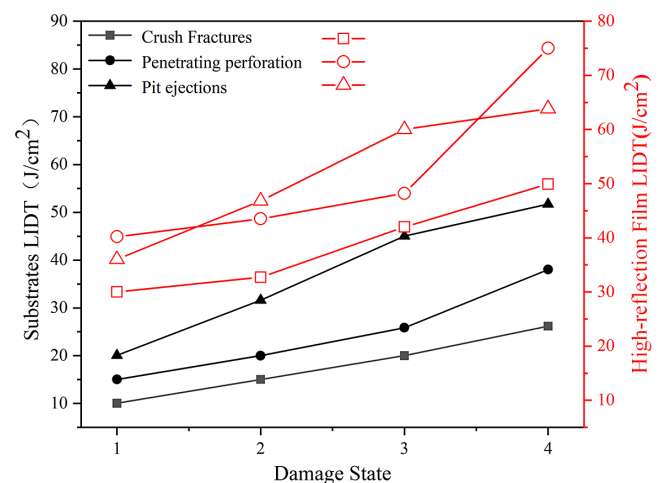
Figure 3. LIDT results for different states in 30\ \mu\text{m} substrates and high-reflection films (1, initial damage morphology; 2, damage to the membrane around the hole; 3, bright spots appearing around the hole; 4, extensive damage centered around the hole).
