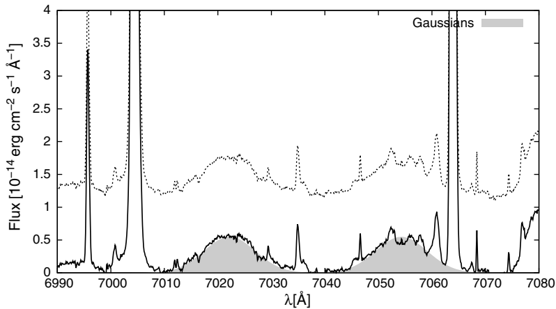
Figure 2. The Raman-scattered C II \lambda\lambda 1036 and 1037 at 7025 and 7052 Å. Our best fits with single Gaussian are shown by gray shaded regions.
