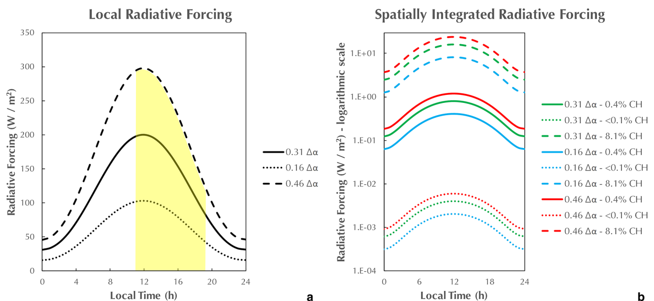
Figure 6. Daily variation of local (a) and spatially integrated (b) radiative forcing induced by cryoconite hole (CH) presence. Different albedo differences ( \Delta\alpha ) refer to the maximum (0.46) and the minimum difference (0.16) of albedo between blue ice and CH, as well as between their average values (0.31). In (b) are also shown the variation of radiative forcing as a function of increasing cover of CH surface over blue ice areas, here calculated from a minimum <0.1% to a maximum of 8.1%, with an average of 0.4%. The yellow area refers to the corresponding span of time during which field spectral measurements were acquired.
