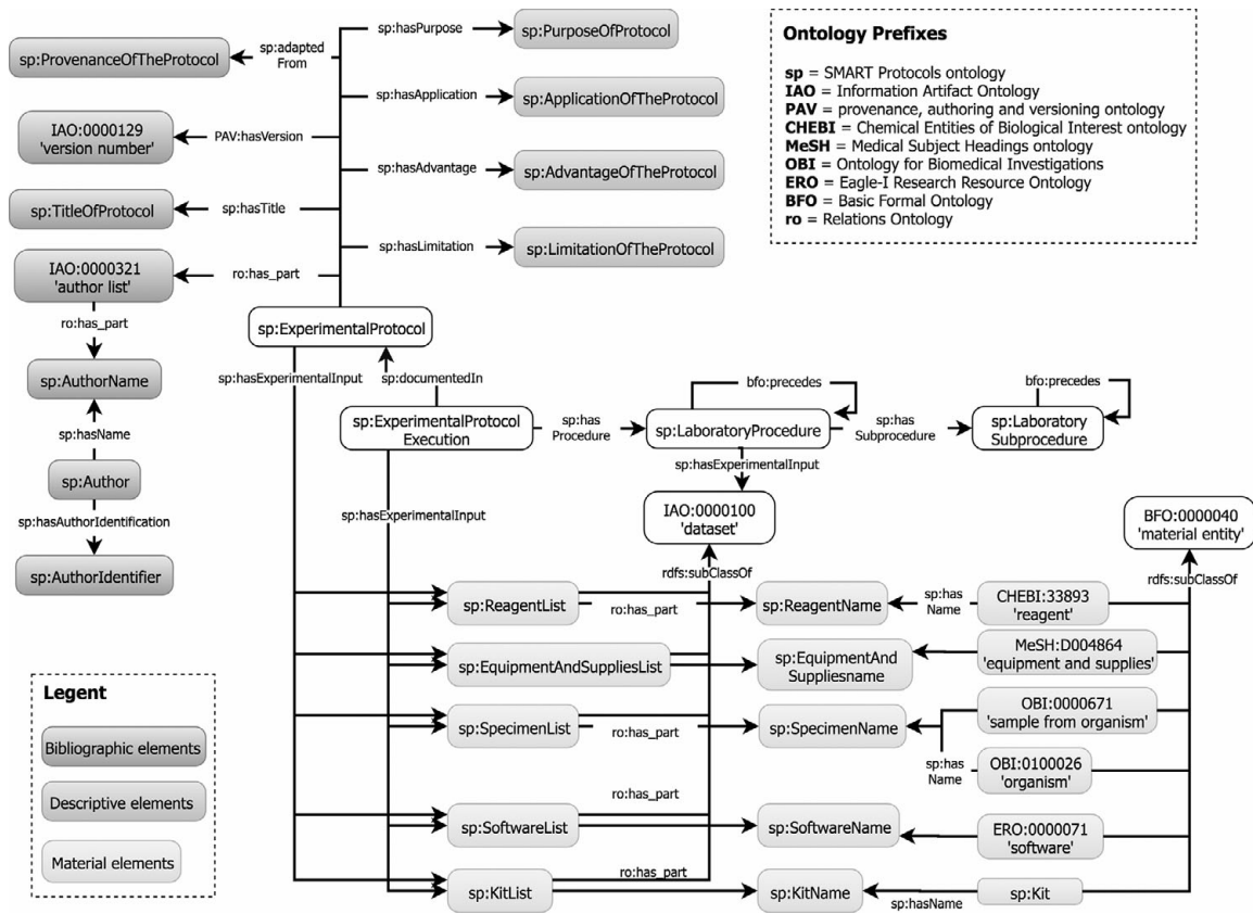
Figure 4.2 Hierarchical organisation of data elements in the SMART Protocols Ontology, sourced from Giraldo et al. 2018 (Image: CC BY 4.0 DEED Attribution 4.0 International).
