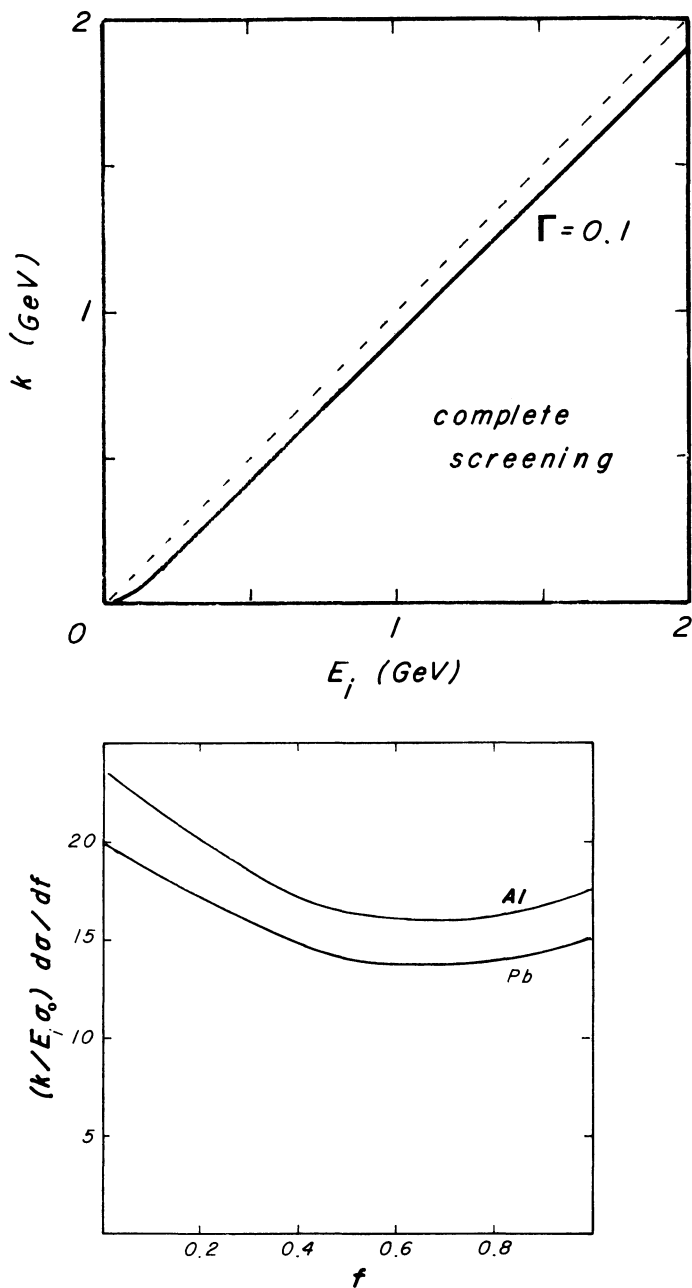
Figure 2.9 (a) The kinematic region of complete screening for bremsstrahlung and the contour for lead with \Gamma = 0.1 . (b) The complete screening bremsstrahlung cross sections for aluminum and lead versus the variable f = k/(E_i - mc^2) .
