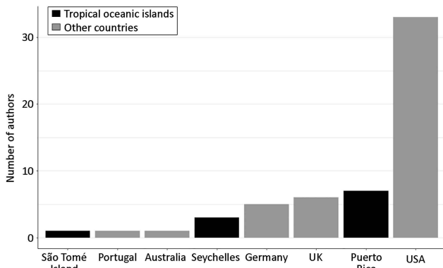
FIG. 3 Locations of the affiliations of authors who published research evaluating amphibian vulnerability to climate and land-use changes on tropical oceanic islands during 1 July 1998–30 June 2022. Note there were no authors from Cuba or The Bahamas in the studies in these countries (Table 1).
