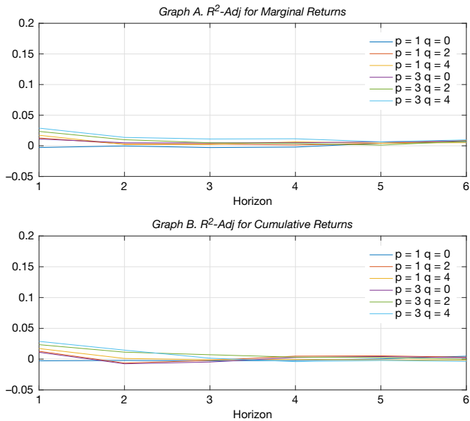
FIGURE 6 Predictability R^2 for ARMA components for RV
