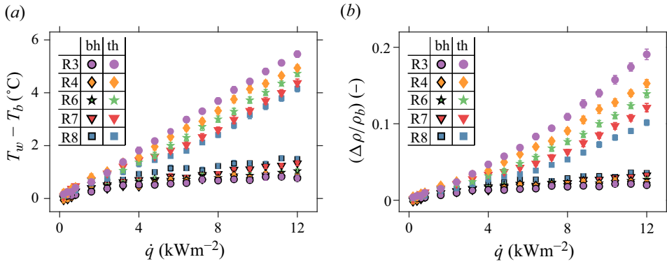
Figure 19. Wall temperature (a) and deduced wall density data (b) for a selection of cases with different nominal Reynolds numbers from figures 4 and 5. Bottom-up (bh) heating data points are shown with black-outlined markers, whereas top-down (th) heating data points are shown with homogenous markers. The data are shown with error bars of \pm 2\sigma .
