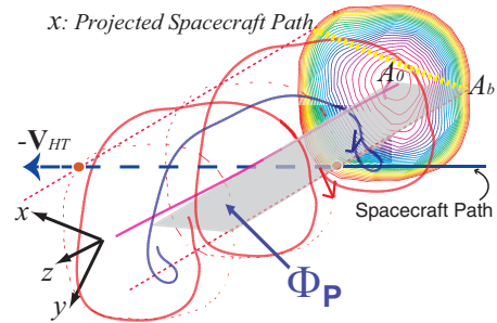
Figure 1. A typical GS reconstruction result of a cylindrical magnetic flux rope. See text for details.
