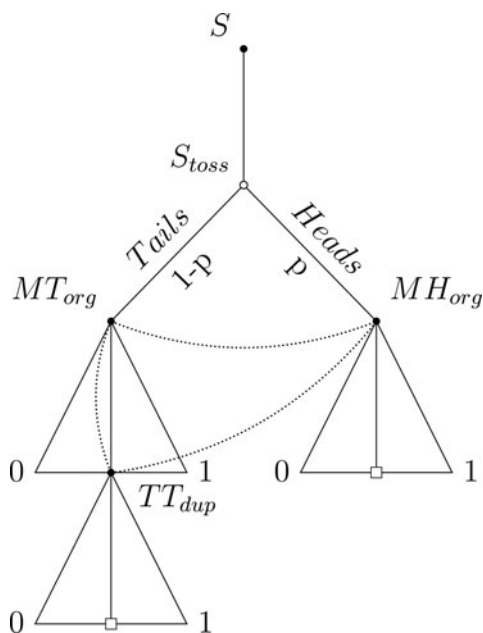
Fig. 2. A model for the duplicating Sleeping Beauty problem with decision nodes of multiple players belonging to a single information set.
