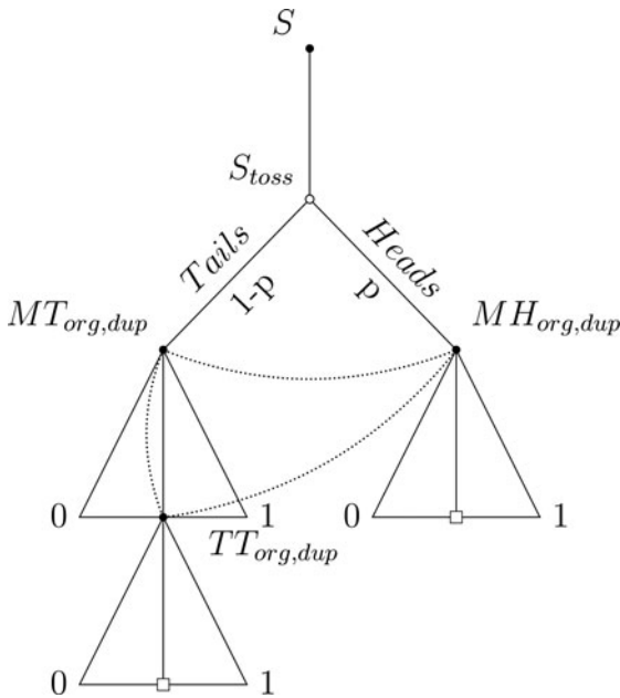
Fig. 3. Multiple agents assigned to the same nodes, where, e.g., MT_{org,dup} means that MT belongs to the original Beauty and the duplicate at the same time.
