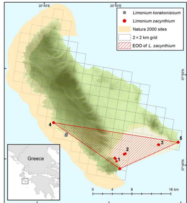
FIG. 1 Distribution of Limonium korakonisicum and Limonium zacyanthium , their area of occupancy (i.e. the number of occupied 2 \times 2 km grid cells), and the estimated extent of occurrence (EOO) of L. zacyanthium . Numbers indicate subpopulations (Lz1, etc.; Table 1).
