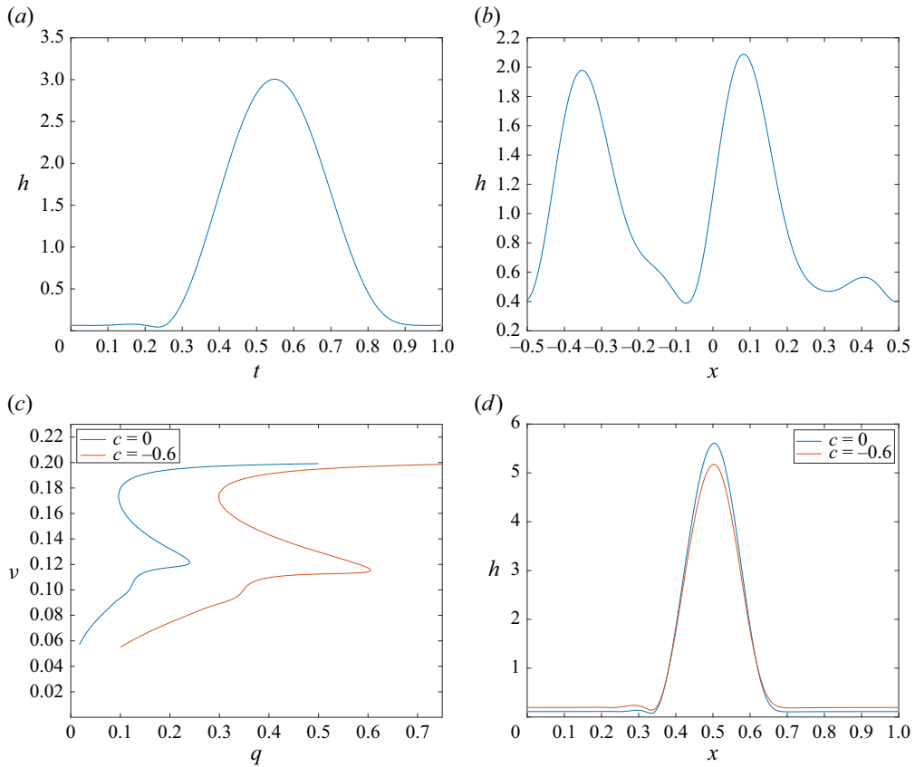
Figure 9. (a) The wave profile for d_1 = 0.8 , d_2 = 0.7 and v = 0.23 . (b) The wave profile for d_1 = 0.8 , d_2 = 0.4 and v = 0.057 . The wave speed is approximately -0.6 . (c) The bifurcation diagrams of travelling wave solutions with fixed mean thickness of 1 for d_1 = 0.8 , d_2 = 0.4 . The wave speeds are -0.6 and 0 . (d) Wave profiles for v = 0.057 on the bifurcation curves in figure 9(c).
