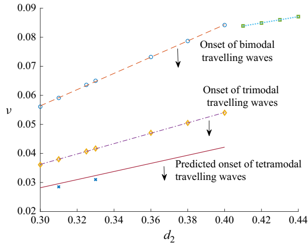
Figure 11. The boundary for the onset of bimodal (the dashed red line and dotted blue line), trimodal (the dashed-dotted line) and tetramodal (the solid line) travelling wave solutions in the d_2 - \nu plane for d_1 = 0.8 . The boundary for the onset of tetramodal travelling waves is predicted by the boundary of bimodal travelling waves by the scaling \nu \rightarrow \nu/2 . The data marked by crosses are obtained numerically.
