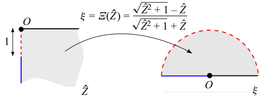
Figure 12. Conformal mappings for solving for \hat{W}(\hat{X}, \hat{Y}) in case (2).
