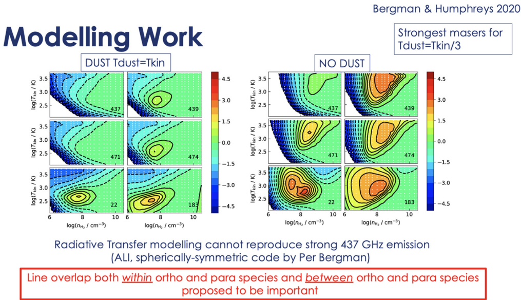
Figure 5. Example modelling results from Bergman & Humphreys (2020). We note that a case with no dust is not realistic for evolved star environments.
