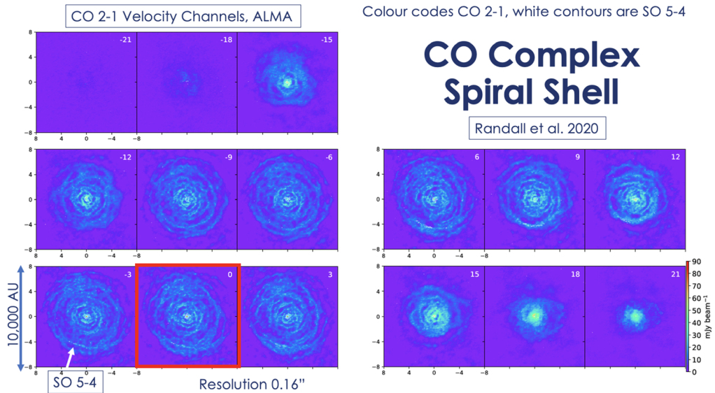
Figure 1. ALMA CO (2-1) observations of GX Mon with 0.16 arcsecond resolution after Randall et al. (2020) . The different panels display velocity channels with that of the systemic velocity (adjusted to zero) outlined by the red box. Colour codes the CO 2-1 emission and white contours are SO 5-4 emission (seen more easily in Figure 2). The SO emission appears to be enhanced in an arc-like structure at about 5 arcseconds south of the central star. At the position of the SO arc, there is also an arc-like filament in the ACS/HST image in the F606W and F814W bands.
