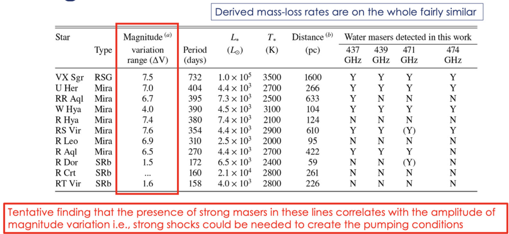
Figure 4. Target list from Bergman & Humphreys (2020) indicating which sources have maser detections. There is a tentative finding that strong masers in these lines correlates with the amplitude of the stellar magnitude variation.
