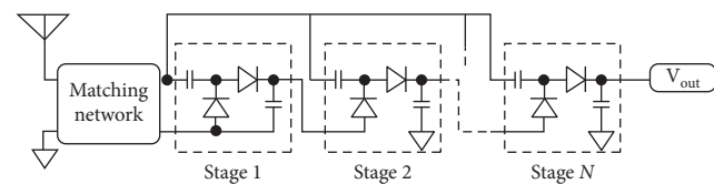
FIGURE 3: Full-wave, N-stage rectifier, Greinacher topology used.
