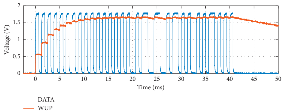
FIGURE 24: Data frame normalization to 1.8 V and wake-up signal generation for the microcontroller.
