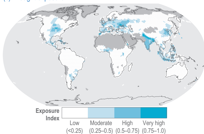
Figure 4.9 | Current global drought risk and its components.
