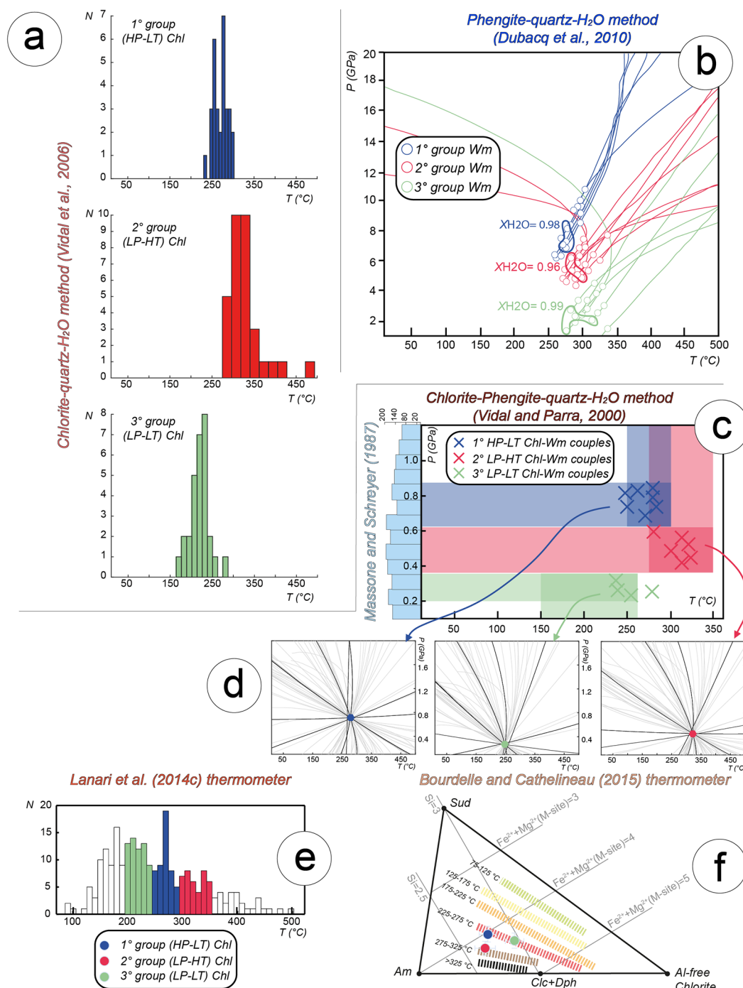
Figure 7. P-T estimate results. (a) Histograms of temperature range of Chl formation belonging to the three groups obtained with Chl-Qz-H 2 O. Each bar represents the counts of each chlorite whose temperature formation falls in a specific range reported along the X-axis. (b) Results of the Phg-Qz-H 2 O barometer. Within the P/T space the equilibrium lines Wm+Qz+H 2 O, together with only the hydration state (empty circles along each line) of white mica changes, are reported for each Wm groups. The XH 2 O values used in the model for each Wm group are also indicated. (c) P/T diagram showing the results of P-T estimates from the Chl-Phg-Qz-H 2 O method. Each cross indicates the pressure and temperature equilibrium condition for a single Chl-Wm couple belonging to the first, the second and the third groups. The blue, red and green boxes mark the temperature and pressure ranges of Chl and Wm formations obtained with the methods reported in a and b. Along the Y-axis, the histogram shows the results of the Massone and Schreyer (1987) barometer. Each bar represents the counting of pressure values for each pixel inside the micro-domain of Fig. 3e. (d) P/T space showing examples of all the independent (black lines) and dependent (grey lines) equilibria obtained with Chl-Phg-Qz-H 2 O for each Chl-Wm couple belonging to the first, the second and the third group. (e) Histograms showing the results of the Lanari et al. (2014c) geothermometer. Each bar statistically represents temperature range values of chlorite formation. (f) Diagram showing the results of the Bourdelle and Cathelineau (2015) geothermometer, where the dashed lines indicate different T ranges. Here, the plot of each average values referred to the different groups of chlorite are reported with their error bars.
