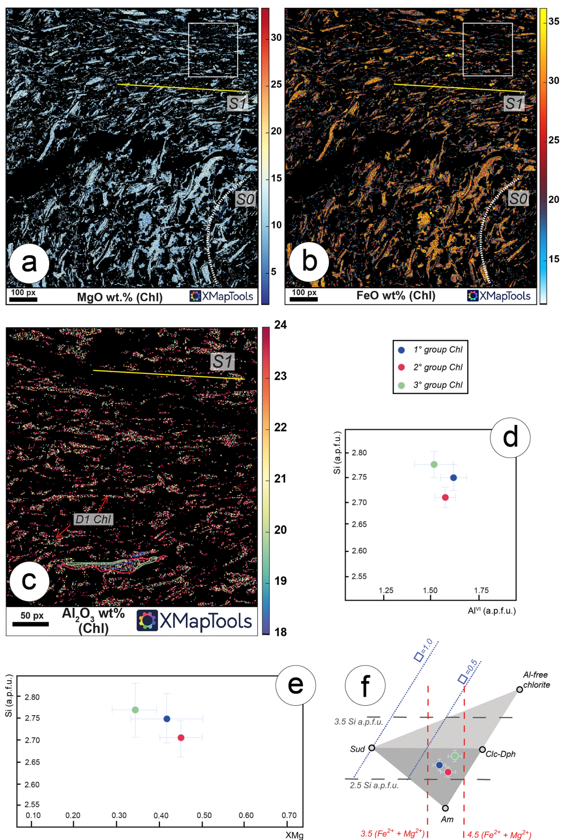
Figure 4. Composition of chlorites in ED208a sample. MgO wt.% (a) and FeO wt.% variation in the microdomain signalled in Fig. 3e. Differences exist between detrital (white dotted line) and syn-metamorphic (yellow line) Chl grains. (c) Enlarged area of the white box of (a) and (b) of the syn-metamorphic Chl (red arrows) grew along the S1 foliation (yellow line). The Al 2 O 3 wt.% variation sheds light the complex mineral chemistry of the neo-formed grains (blue, red and green areas) corresponding to first, second and third groups (see the text). (d) Al VI /Si and (e) XMg/Si plots referred to the average compositions of the three groups of Chl detected along the S1 foliation are reported with their error bars. (f) Octahedral Fe 2+ + Mg 2+ (apfu, red dashed lines) content vs. Si (grey dashed lines) diagram (according to Bourdelle and Cathelineau, 2015). The blue dotted lines show the octahedral vacancy (blue empty squares) values. The four Chl end-members are also reported.
