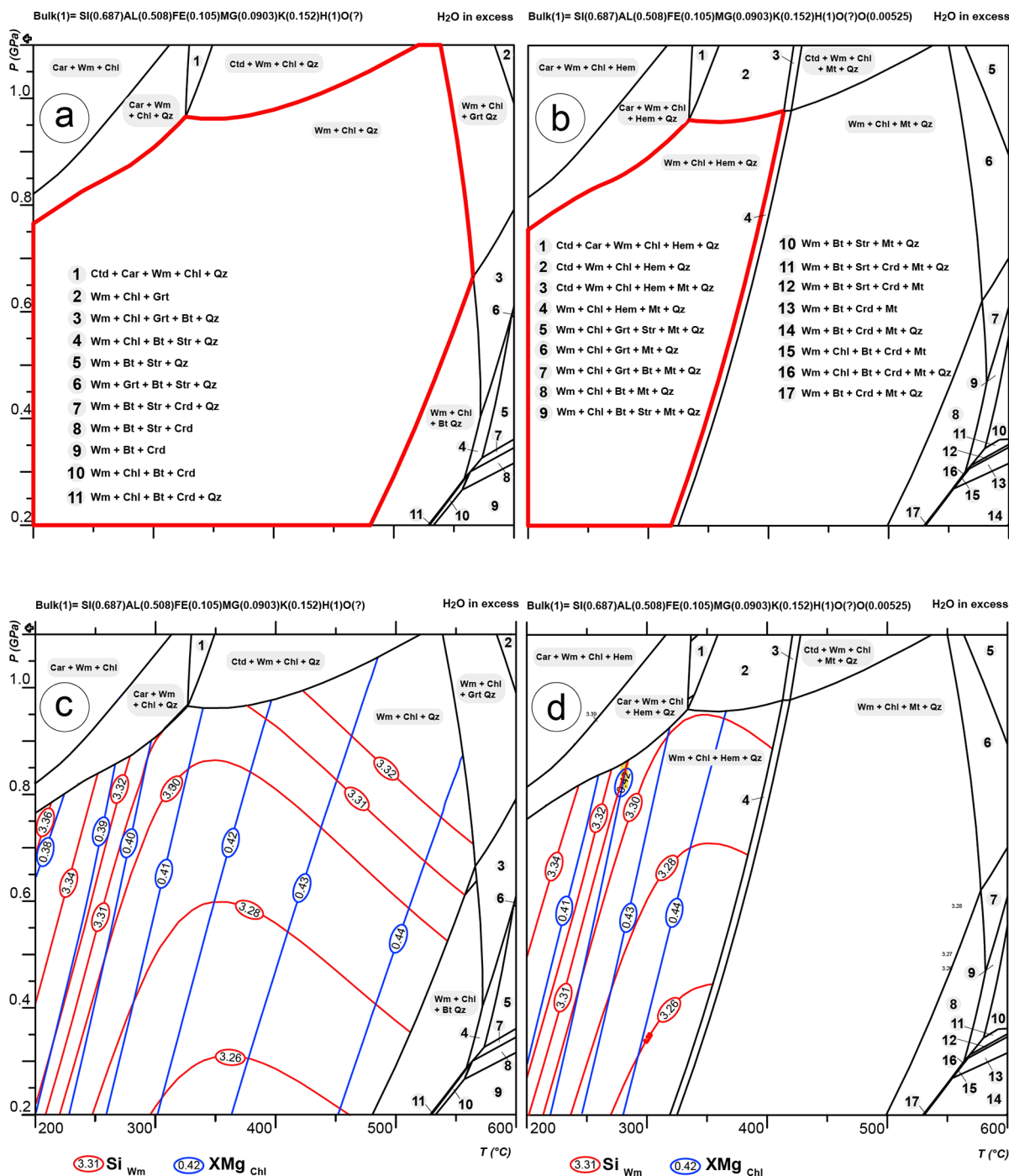
Figure 6. Isochemical phase diagrams related to the micro-domain within the white box of Fig. 3e. (a) Phase diagram with \text{FeO}_{\text{tot}}=\text{Fe}^{2+} . (b) Phase diagram where 10% of \text{FeO}_{\text{tot}}=\text{Fe}^{3+} . Black lines mark the boundary between different stability field, whereas the red ones indicate the field where the observed mineral assemblage is found to be stable. (c, d) Isochemical phase diagrams contoured for Si (Wm) and XMg (Chl) isopleths. The LBC is reported in moles of elements at the top of the diagrams. In the grey boxes, the stable mineral assemblages relate to the different fields are indicated. The yellow area indicates the P/T space of (d) in which the measured value of Si and XMg (for Wm and Chl, respectively) match with that predicted by the model. At the bottom of each diagram, the contour legend is reported and the numbers inside the ellipses represents values of the related observed isopleth. Car: Carpholite; Ctd: Chloritoid; Grt: Garnet; Bt: Biotite; St: Staurolite; Crd: Cordierite; Hem: Hematite; Mt: Magnetite.
