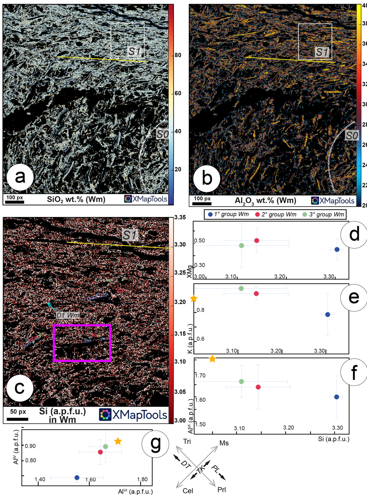
Figure 5. Compositions of Wm in sample ED208a. (a) \text{SiO}_2 wt.% and (b) \text{Al}_2\text{O}_3 wt.% variation in the microdomain of Fig. 3e. Differences exist between detrital (white dotted line) and syn-metamorphic (yellow line) Wm grains. (c) Enlarged area of the white box of (a) and (b) of the syn-metamorphic Wm (light blue arrow) grew along the S1 foliation (yellow line). The Si content variation outlines a complex mineral chemistry of the syn-metamorphic Wm (blue, red and green areas) corresponding to first, second and third groups (see the text). The purple box indicates the Chl the location of chlorite crystal shown in Fig. 4c. (d) XMg/Si, (e) K/Si, and (f) \text{Al}^{\text{IV}} /Si plots refer to the average composition of the three groups of Wm detected along the S1 foliation and include the related error bars. The orange stars indicate the theoretical compositional of muscovite. (g) \text{Al}^{\text{IV}} / \text{Al}^{\text{VI}} plot (according to Bousquet et al. , 2002). The grey arrows indicate the solid solution trend of Wm, while the black arrows indicate the main substitution (TK: Tschermak; DT: Di-trioctahedral; PL: Pyrophyllitic).
