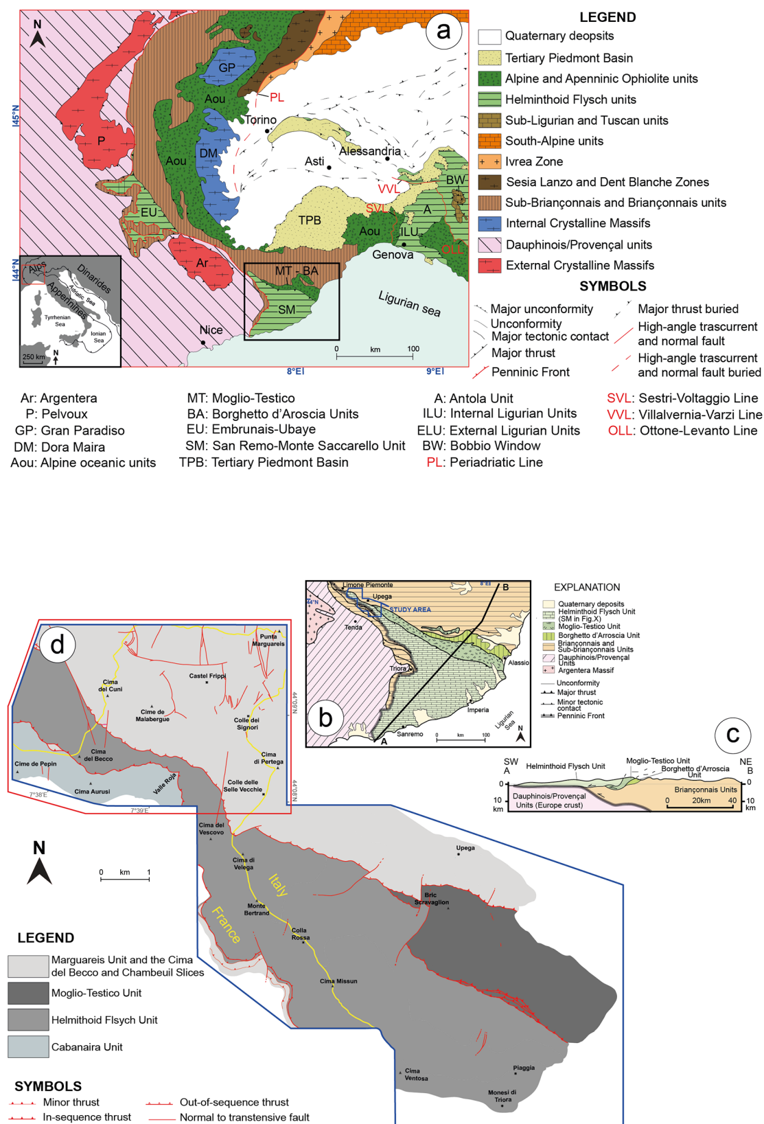
Figure 1. (a) Geological scheme of the Western Alps-Northern Apennines (modified and re-drawn from Molli et al. , 2010 and Sanità et al. , 2021a). (b) Close-up of the Western Ligurian Alps (black box of a) with the related geological cross-section (c) modified by Bonini et al. (2010). (d) Simplified geological sketch (blue box of b) of the boundary between Maritime and Ligurian Alps.
