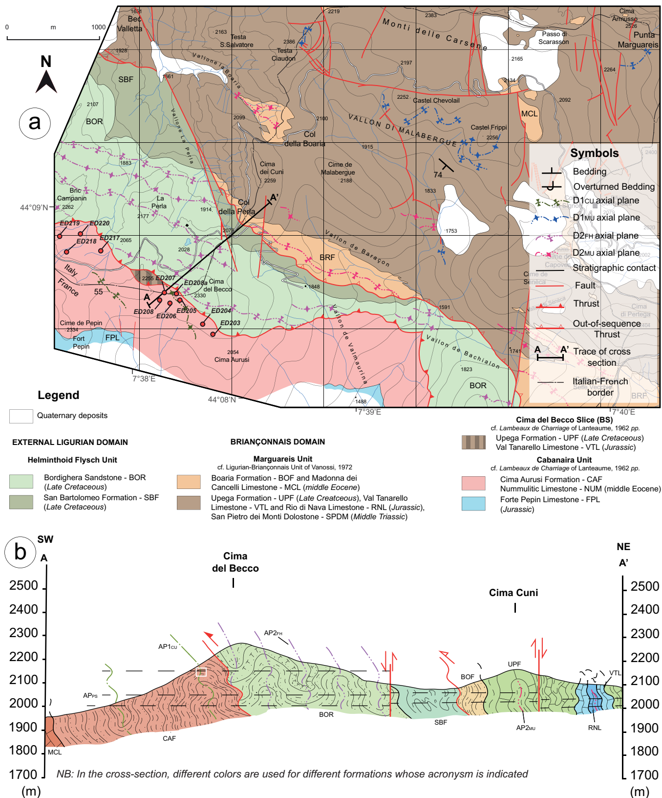
Figure 2. (a) Geological map (modified from Sanità et al. , 2021a and 2021b) of the Marguareis Massif (red box of Fig. 1d) with the related geological cross-section (b). In the map the locations of samples are reported (red dots).
