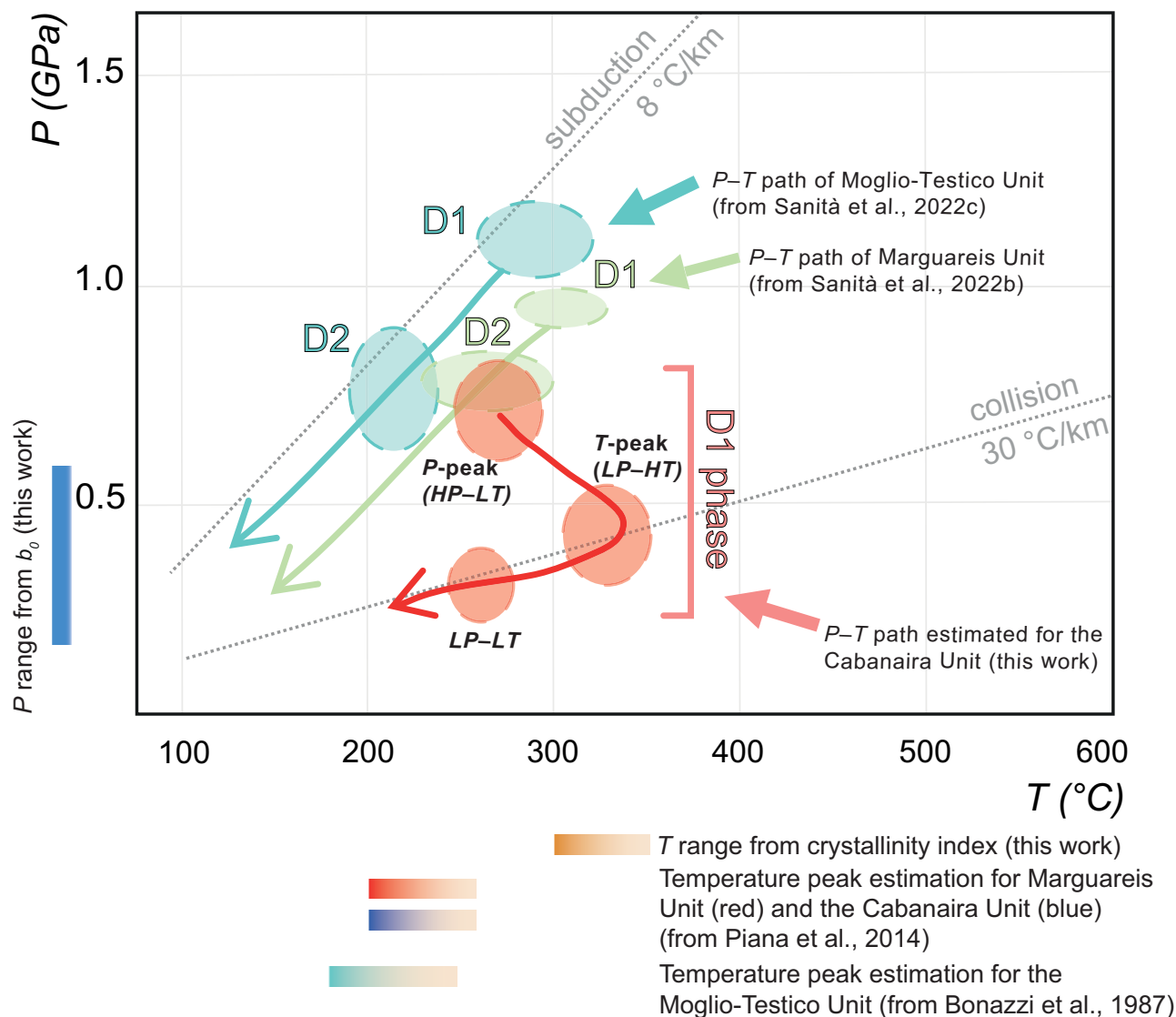
Figure 9. Diagram showing the P - T path of the Cabanaira Unit constrained in this work. The paths estimated for the Marguareis and Moglio-Testico Unit are also represented (data from Sanità et al. , 2022b; 2022c). The geothermal gradients typical of subduction and collision setting are also shown. Along the X-axis the T ranges extrapolated by means Illite Crystallinity Index for the Marguareis (red rectangular bar data from Piana et al. , 2014), Cabanaira (blue rectangular bar from Piana et al. , 2014; orange rectangular bar from this work) and the Moglio-Testico (light blue rectangular bar from Bonazzi et al. , 1987) Units are reported. The shaded effect indicates that the upper limit of the range is poorly constrained with this method. Along the Y-axis the P range yielded from b_0 measurement (this work) are reported. The length of rectangular boxes represents the range of temperature and pressure estimates.
