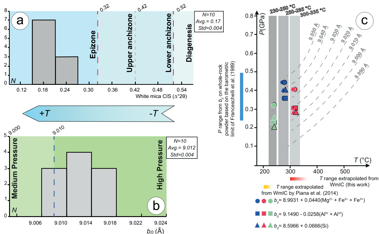
Figure 8. Crystallochemical indices distribution. (a) WmIC distribution. (b) b_0 cell parameters distribution from XRD patterns. (c) b_0 values calculated using the Verdecchia et al. (2019) spreadsheet. The grey rectangular boxes represent the three T ranges independently obtained with thermobaric methods. Along Y- and X-axes the crystallochemical index distribution (coloured rectangular bars) obtained using the XRD pattern analysis is reported. The T ranges calculated by Piana et al. (2014) are reported (yellow rectangular bar along the X-axis). The shaded effect indicates that the upper limit of the range is poorly constrained with this method. The triangles, circles and squares contoured in black are referred to the calculations in which 10% of ferric iron is considered.
