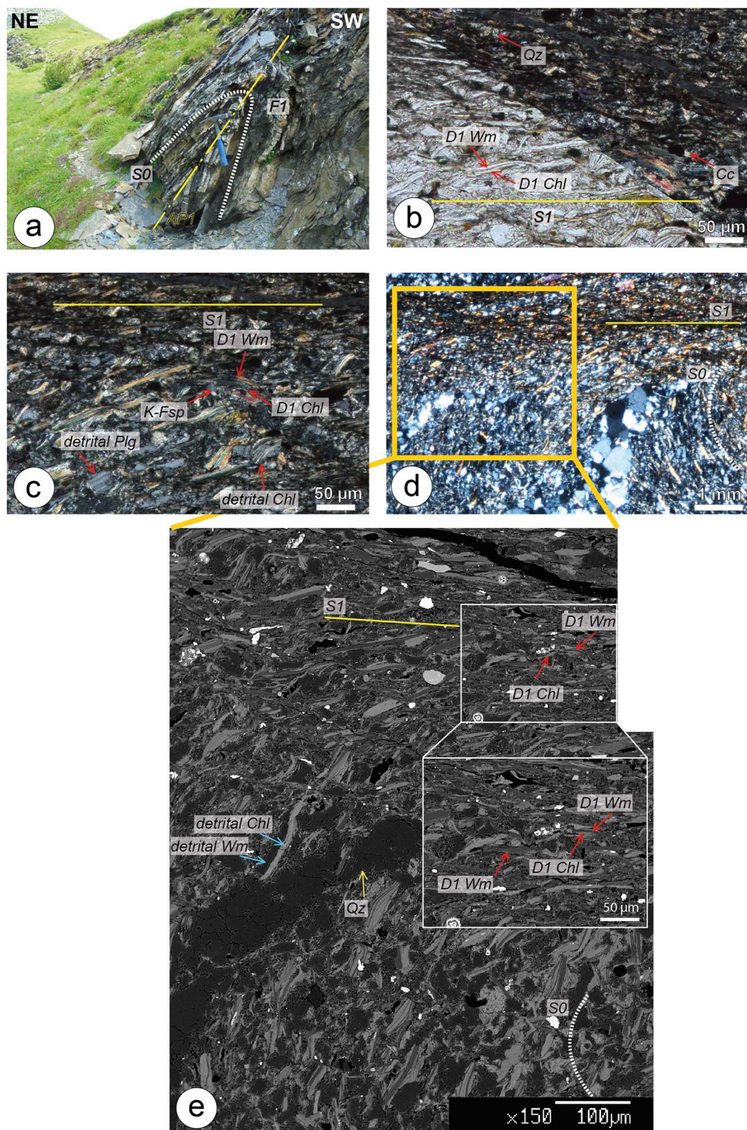
Figure 3. Macro- to micro-scale D1 phase-related structural features. (a) F1 fold system in the Cabanaira Unit (white box of Fig. 2b). (b, c) S1 (yellow line) slaty cleavage (bottom left of b: plane polarized light, top right of b and c: crossed polarized light) marked by syn metamorphic Wm and Chl and Qz in textural equilibrium. Detrital grains of plagioclase and chlorite (c) can be observed. (d) Microphotograph of F1 hinge-zone where clear cross-cutting relationships between S1 (yellow line) and bedding (S0, white dashed line) are shown. (e) BSE image of the micro-area investigated to perform the P - T estimates (orange box of d). The white box represents the area where the local bulk composition was extracted to perform forward and inverse thermodynamic modelling. Along the S0 (white dashed line), detrital Wm and Chl (blue arrows) are indicated. Along the S1 (yellow line) neo-formed Wm and Chl crystals (red arrows in the white boxes) are present.
