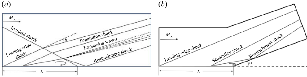
Figure 2. Computational domains and schematics of (a) incident shock flow and (b) compression corner flow.
