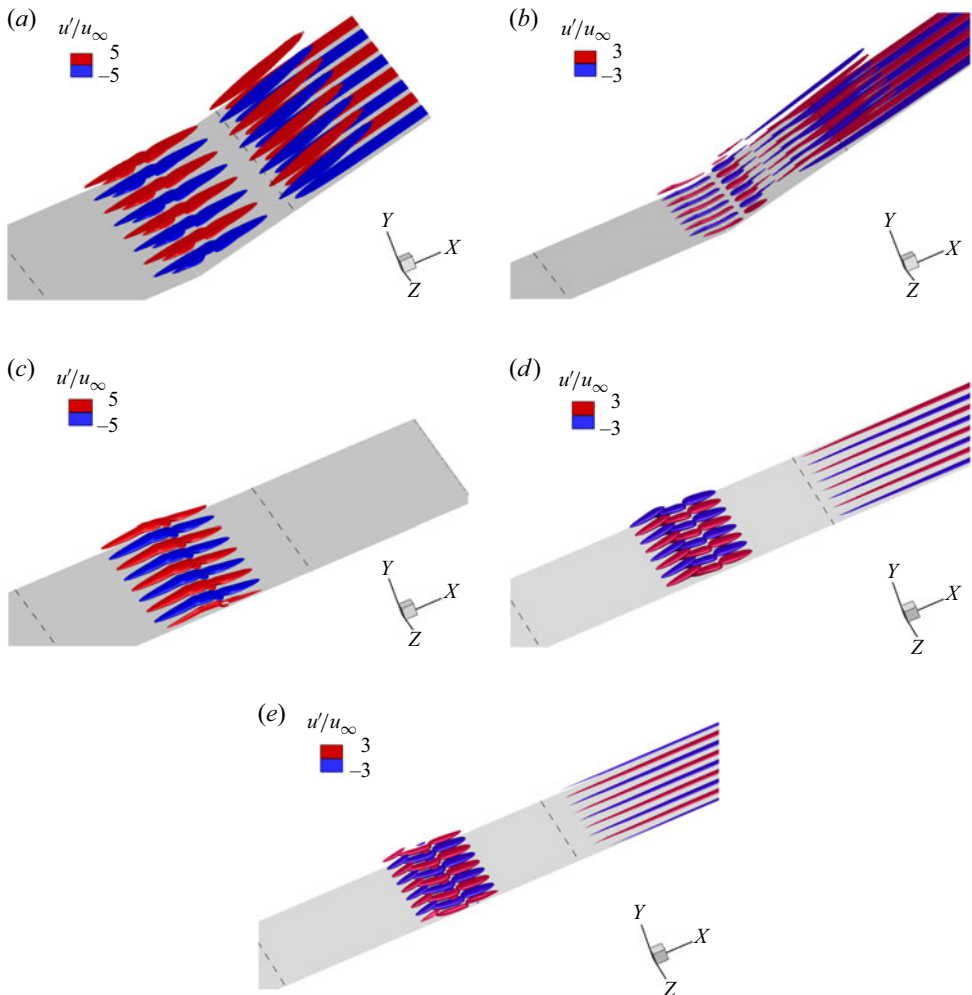
Figure 37. Isosurfaces of the real parts of eigenfunctions u' for 10.2° compression ramp flow at (a) \beta L = 22 (S mode) and (b) \beta L = 58 (S-O mode), and for 6.5° incident shock flow at (c) \beta L = 34 (S mode), (d) \beta L = 72 (O mode) and (e) \beta L = 79 (O-S mode).
