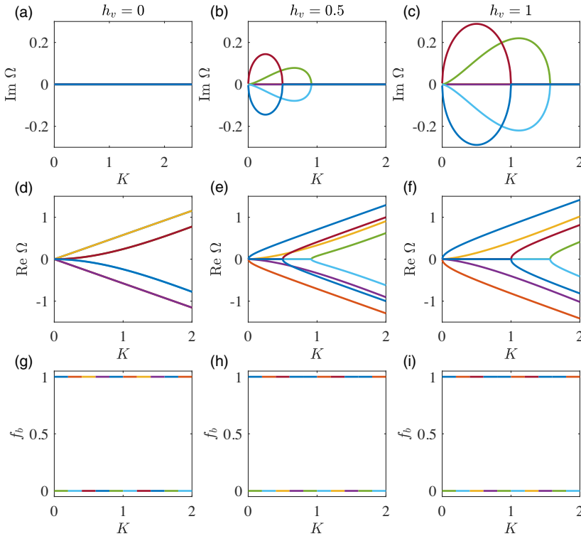
FIGURE 1. The imaginary ( a – c ) and real ( d – f ) parts of modulational frequency \Omega versus modulatory wavevector K at m = a = h_b = h_c = 0 and St = 10^5 for h_v = 0 ( a,d ), h_v = 0.5 ( b,e ) and h_v = 1 ( c,f ). The magnetic-energy fraction f_b \doteq b^2/(v^2 + b^2) of the corresponding eigenmodes are given in panels ( g )–( i ). The frequencies are given in units of the inverse turnover time \tau^{-1} and wavevectors are given in units of the inverse characteristic eddy size l^{-1} .
