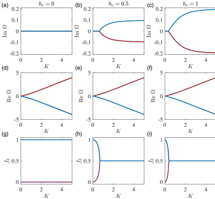
FIGURE 3. The imaginary (a–c) and real (d–f) parts of modulated frequency \Omega normalised to \tau^{-1} at m = 1 , a = h_b = h_v = 0 and St = 10^5 for h_c = 0 (a, d), h_c = 0.5 (b, e) and h_c = 1 (c, f). The magnetic energy fraction f_b \doteq b^2/(v^2 + b^2) of the corresponding eigenmodes is presented in panels (g)–(i). The frequencies are given in units of the inverse turnover time \tau^{-1} and wavevectors are given in units of the inverse characteristic eddy size l^{-1} .
