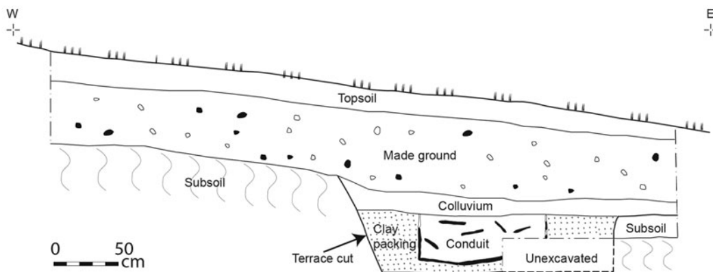
FIG. 7. South facing section drawing of Trench 1 showing the aqueduct terrace cut and shape of wooden conduit.
