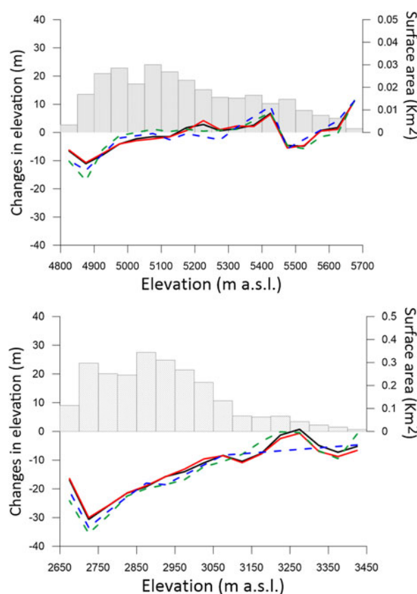
Fig. 10. Hypsometry (gray histogram) and changes in elevation vs altitude for (a) Glaciar Antisana 15α over the period 1997–2009; and (b) Glacier de Saint-Sorlin over the period 2003–2014. The variation in elevation was averaged for each 50-m elevation band. The changes in elevation extracted by the different approaches are shown: SeqDEM (solid black line), profiles along the central flowline (green dashed line) and perpendicular (blue dashed line) to the central flowline and geo-statistical analysis (red line).
