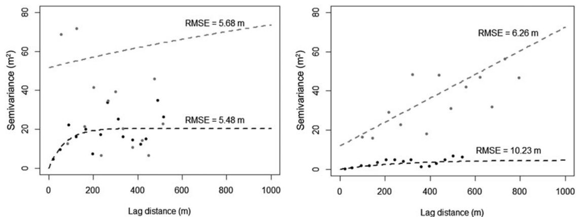
Fig. 8. Experimental semi-variogram and fitted exponential model for the topographic profiles measured for the two glaciers (Antisana 15α on the left and Saint-Sorlin on the right): black circles and black dashed line correspond to perpendicular profiles and gray circles and gray dashed line correspond to profiles along the central flowline. The RMSE from the cross-validation process for the profiling method is given in each graph.
