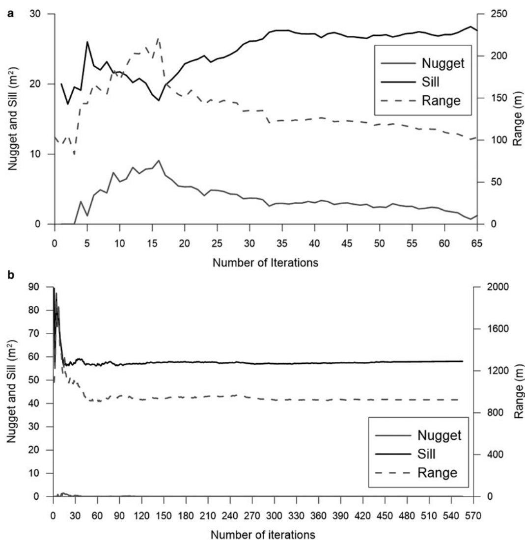
Fig. 6. Changes in the parameters of the semi-variogram model as a function of the number of iterations for (a) Glaciar Antisana 15α and (b) Glacier de Saint-Sorlin.
