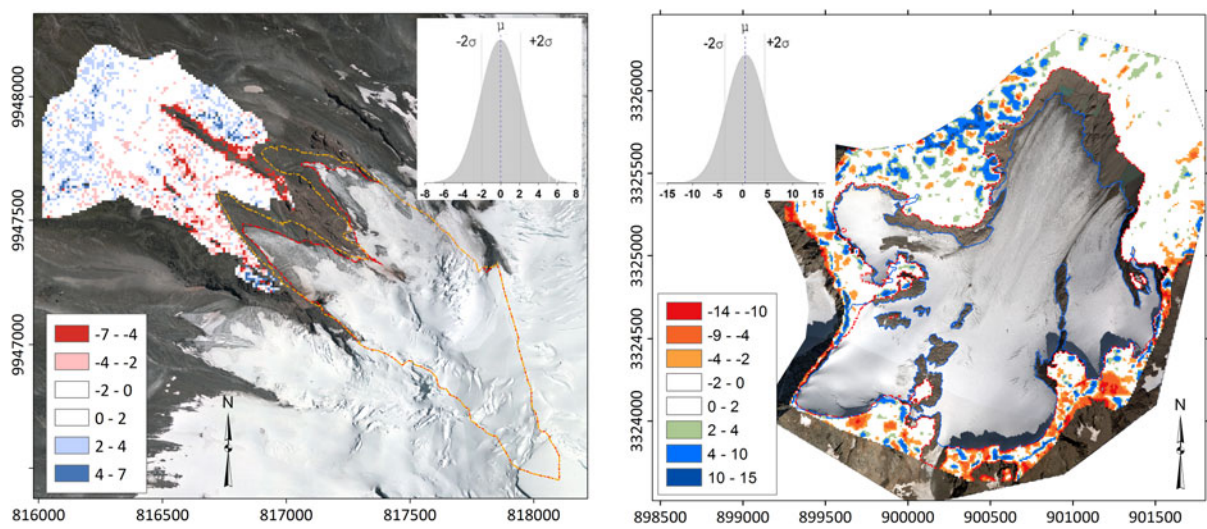
Fig. 3. Surface-elevation changes (m) on the glacier foreland: for Glaciar Antisana 15α [DEM1997\DEM2009] on the left, and Glacier de Saint-Sorlin [DEM2008\DEM2014] on the right, with respectively 5131 and 18 700 pixels (spatial resolution = 10 m). The normal distribution, mean and two std dev. of the elevation changes are shown in the inset graph.
