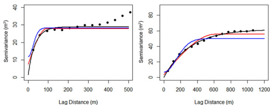
Fig. 5. Experimental semi-variogram (black circles) and fitted theoretical models: spherical (red), exponential (black), and Gaussian (blue); for the two glaciers (Antisana 15α on the left and Saint-Sorlin on the right). The parameters of each theoretical semi-variogram are listed in Table 4.
