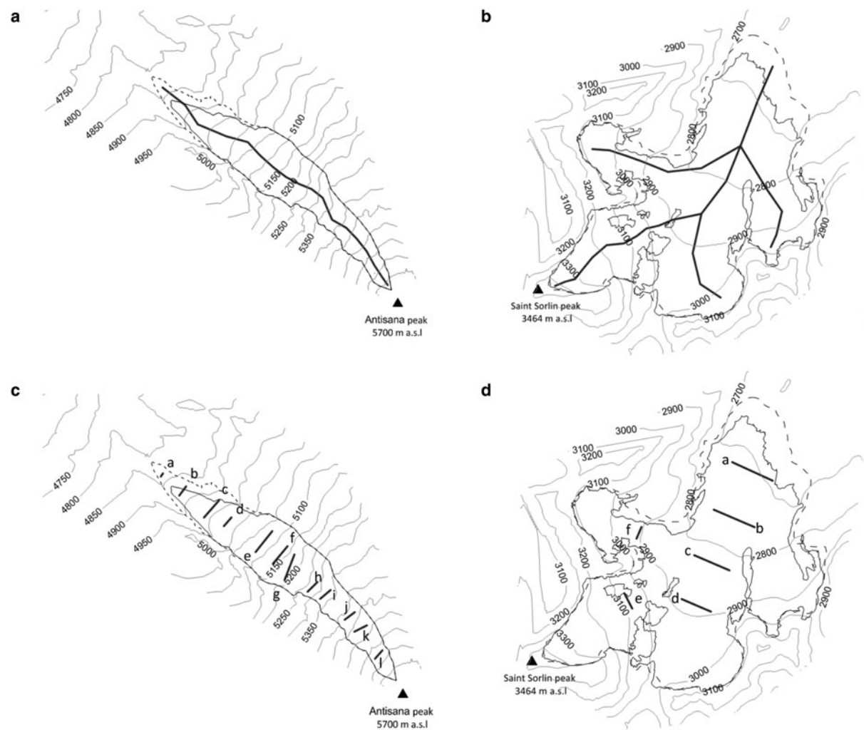
Fig. 4. Topographic profiles along (a and b) and perpendicular (c and d) to the central flowline used to compute changes in thickness for Antisana 15α and Saint-Sorlin glaciers using geodetic measurements. The gray dashed lines are the outlines of the glacier in September 2009 and August 1997 for Antisana 15α and the outlines of the glacier in September 2014 and August 2003 for Saint-Sorlin.
