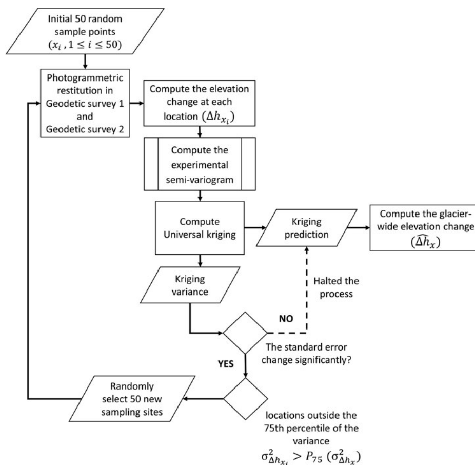
Fig. 2. Schematic overview of the SSD method.
