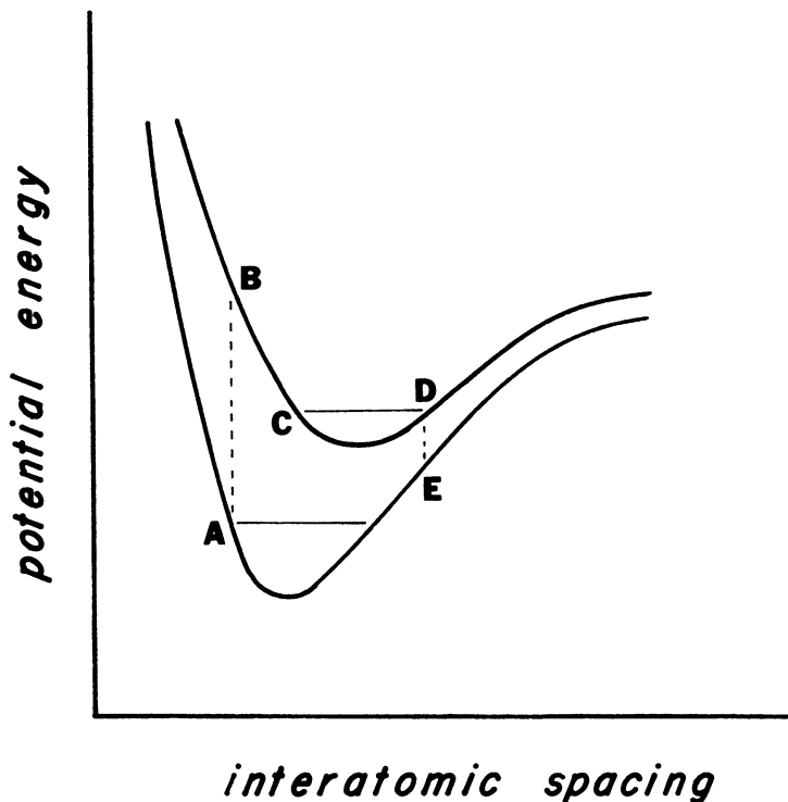
Figure 7.2 Molecular potential energy versus interatomic spacing.
