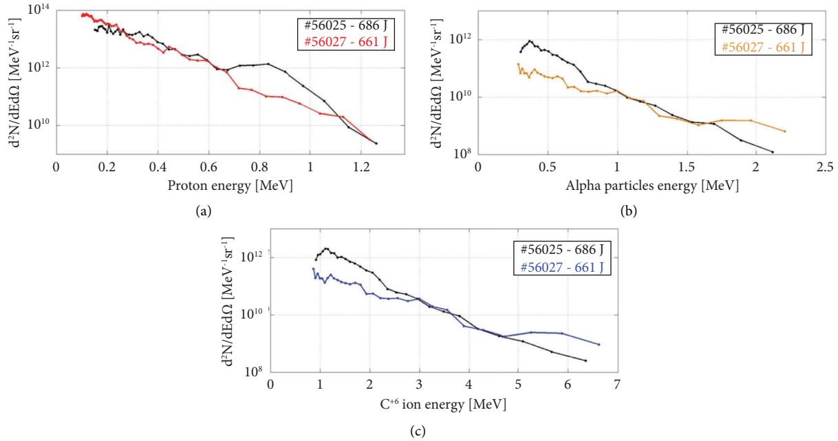
FIGURE 7: Spectra obtained for two typical shots (shot #56025 indicated by black curves and shot #56027 indicated by colored curves). (a) Proton traces. (b) A/Z = 2 traces assuming that the signal is generated by \alpha particles. (c) A/Z = 2 traces assuming that the signal is generated by C^{6+} ions.
