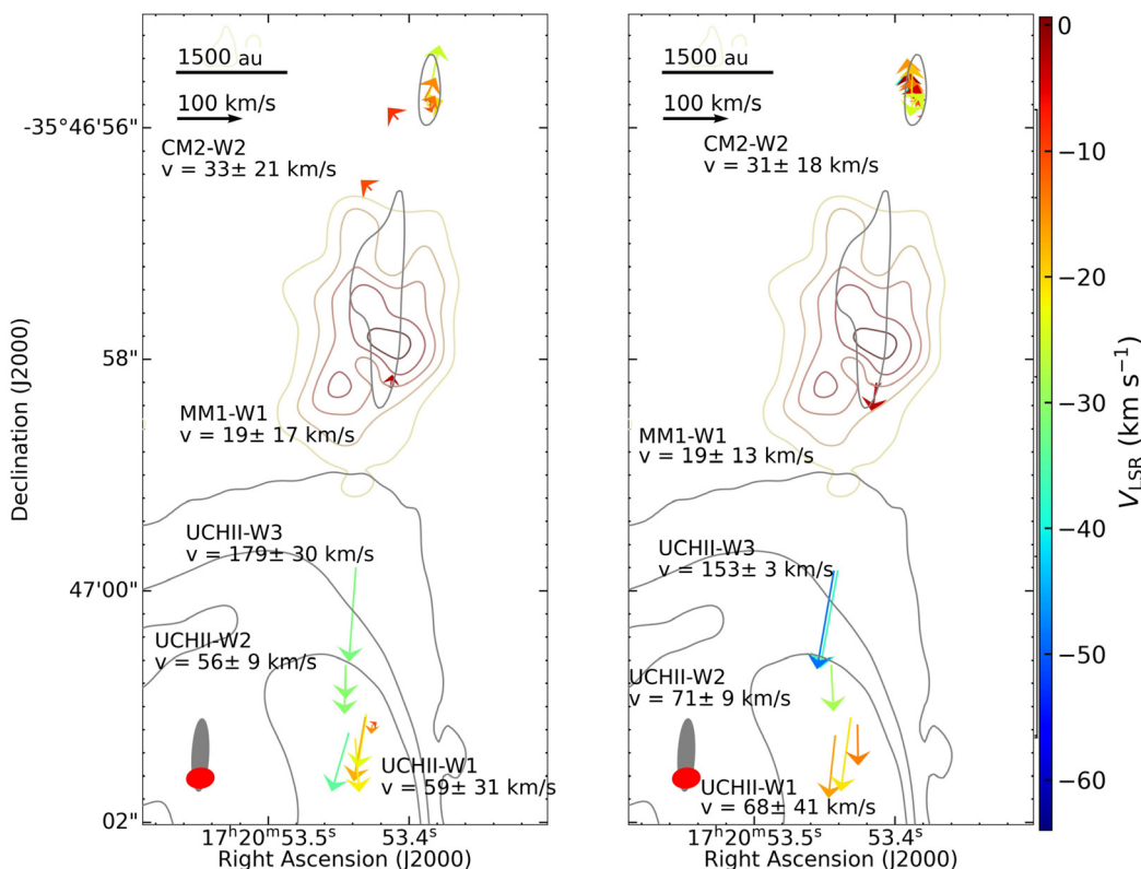
Figure 2. Proper motions of water masers in NGC6334I before (2014.7 – 2015.3) and during (2015.9 – 2016.2) the accretion burst. The mean velocities of each region is shown in black text. The brown contours represent the ALMA 1.3 mm continuum and the grey contours the JVL 5 cm continuum, as in Brogan et al. (2018) .
